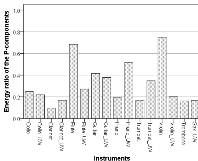
Fig. 4. Energy ratio of the P-components for different instrument samples from the instrument recognition tests MACarena and UW-CAMP. ( j=15 , STFT 185 ms)
