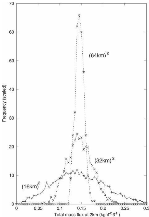
FIG. 1. Frequency plot of total convective mass flux per unit area (at a height of 2 km) obtained from a CRM simulation (Cohen and Craig 2006) of radiative-convective equilibrium. The total mass flux is computed for different-sized areas and binned into intervals of 0.01 \text{ kg m}^{-2} \text{ s}^{-1} . Data are taken from the established equilibrium state only using 340 times over 2 days. The vertical axis is scaled to account for the larger number of suitable areas that become available as the unit-averaging area is reduced in size.
