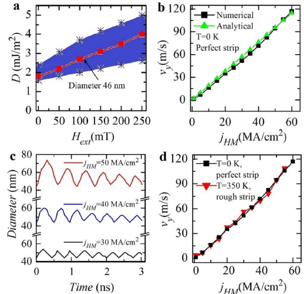
Figure 3 | Skyrmion racetrack memory at zero bias field. (a), Phase diagram (Interfacial DMI parameter vs. external field) of the skyrmion stability. The colored part highlights the region where the skyrmion is stable and the red curve points out the values of D and H_{ext} for which the skyrmion diameter is 46 nm. (b), Skyrmion velocity as a function of the current calculated by micromagnetic (black curve) and analytical computations (green line) (the parameters can be found in Supplementary Material S1). (c), Time domain evolution of the skyrmion diameter during the transient breathing mode at three different values of the j_{HM} , 30 MA/cm 2 (black curve), 40 MA/cm 2 (blue curve) and 50 A/cm 2 (red curve). (d), A comparison of skyrmion velocity as a function of the current for an ideal strip ( T = 0 K) and a rough strip and room temperature.
