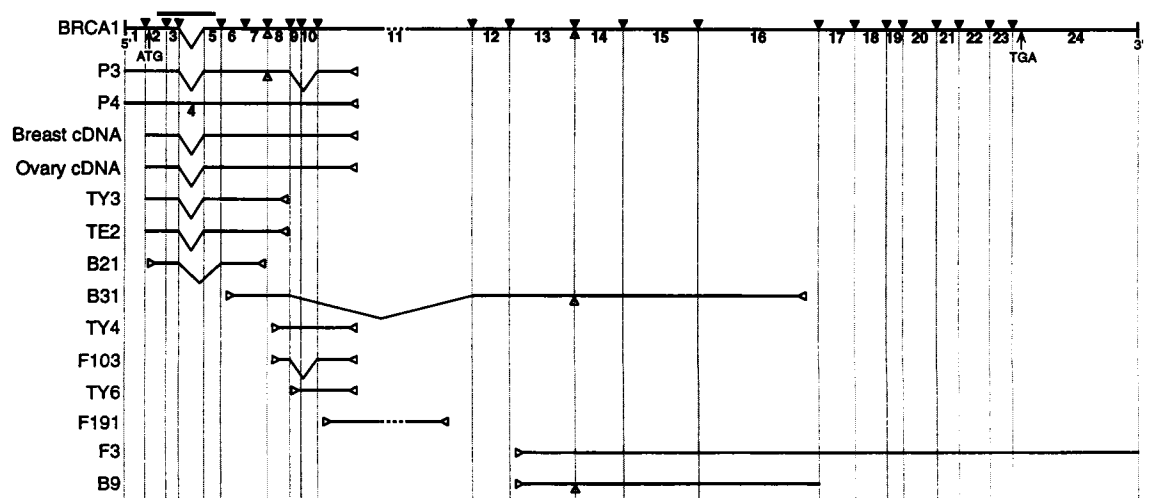
Fig. 3. Diagram of BRCA1 mRNA, showing the locations of introns and the variants of BRCA1 mRNA produced by alternative splicing. The top cDNA ( BRCA1 ) is the composite used to generate the protein sequence in Fig. 2. Intron locations are shown by filled triangles, and the exons are numbered below the composite cDNA. Alternative mRNAs identified as cDNA clones or in hybrid-selection experiments are shown below the composite. The start codon (ATG) and stop codon (TGA) are indicated. The zinc finger region is denoted by a double line. "V" lines connecting exons indicate the absence of internal exons. All exons are drawn proportionally except exon 11 (indicated with a dotted line). Upward-pointing unfilled triangles show the position of a single codon (CAG) found at the start of exons 8 and 14 in some cDNAs. Leftward- and rightward-pointing unfilled triangles represent partial exons in some cDNAs. P3 and P4 are cDNA clones isolated from a placental cDNA library;
