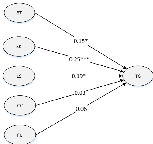
Fig. 2. Path Coefficients for the Proposed Structural Model
