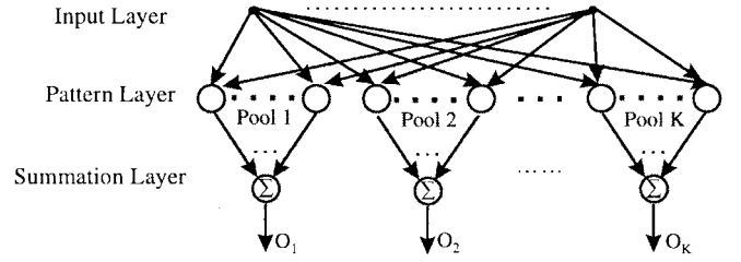
Fig. 3. The structure of PNN.
