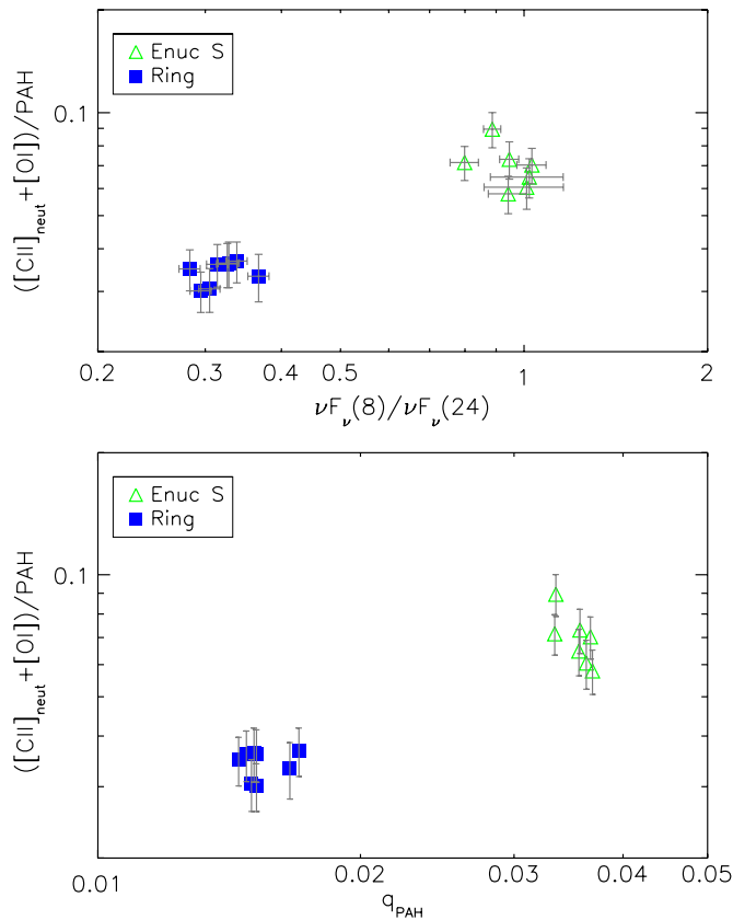
Figure 13. Upper: plot of the ([\text{C II}]158\mu\text{m} + [\text{O I}]63\mu\text{m})/\text{PAH}(5.5\text{--}14\mu\text{m}) ratio as a function of F_{\nu}(8\mu\text{m})/F_{\nu}(24\mu\text{m}) as traced by Spitzer -IRAC bands for the regions defined in Section 3.3. Lower: plot of the ([\text{C II}]158\mu\text{m} + [\text{O I}]63\mu\text{m})/\text{PAH}(5.5\text{--}14\mu\text{m}) ratio as a function of the PAH mass abundance q_{\text{PAH}} , calculated using the dust emission models of Draine & Li (2007).
