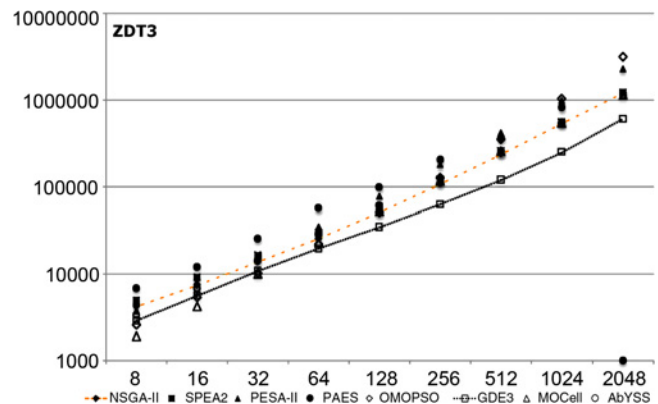
Fig. 6. Number of evaluations when solving ZDT3.
