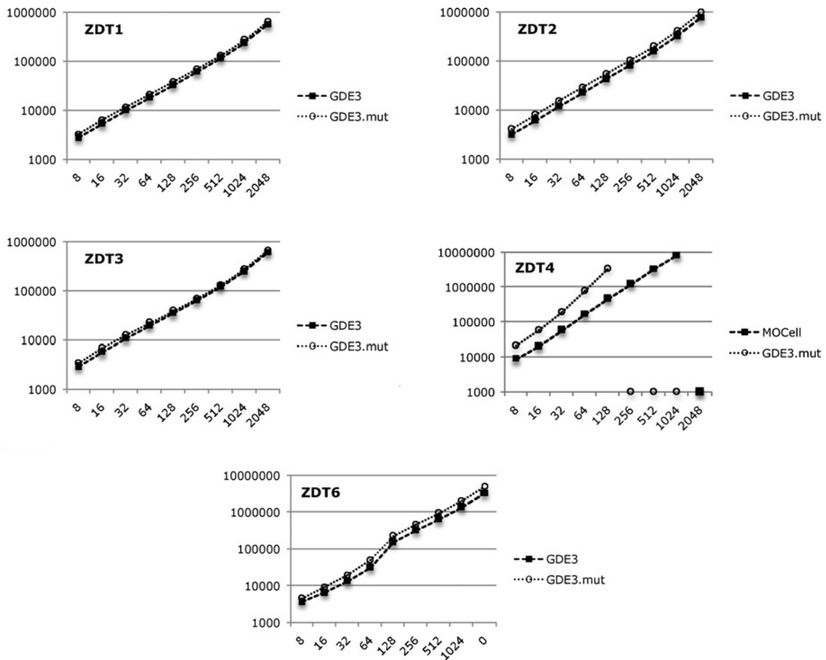
Fig. 14. Results of GDE3 with polynomial mutation on the ZDT problem family.
