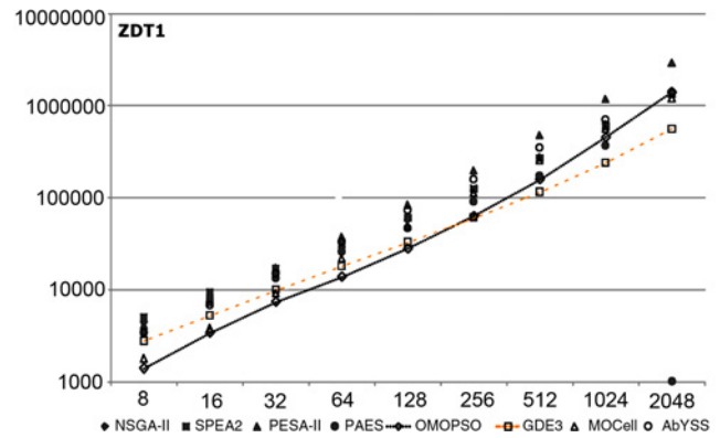
Fig. 4. Number of evaluations when solving ZDT1.
