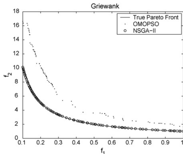
Fig. 9. OMOPSO solving Griewank's test problem.
