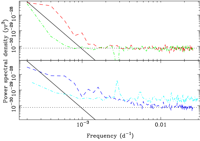
Figure 6. Power spectra averaged over the 20 simulated pulsars for S_{tt} (dashed line) and S_{de} (dot-dashed line). S_{ie} at 200 ns (dashed line) and S_{sw} (dot-dashed line) are shown in the bottom panel. In both panels the expected power spectral density for a GWB with A = 10^{-15} is shown as the black solid line. The power spectral density corresponding to 100 ns of white noise is indicated as the black dotted line.
