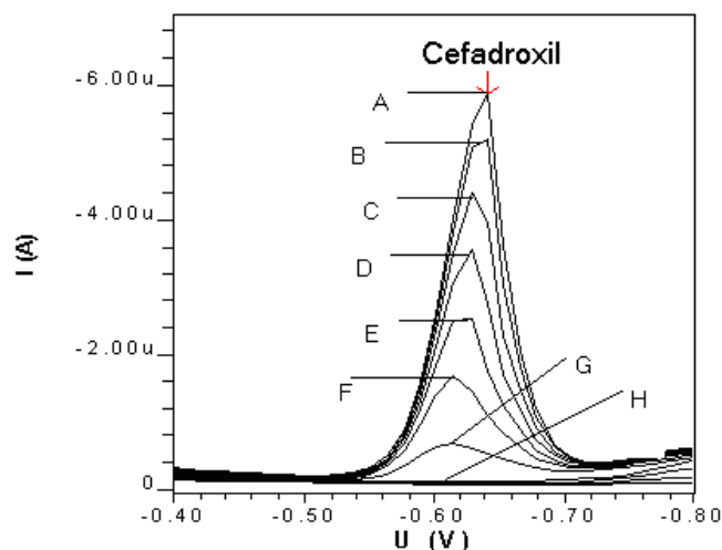
Figure 6. AdSV voltammogram for cefadroxil in the presence of 5 \times 10^{-6} mol L -1 Cu(II) in B-R buffer pH=9.5, T_{acc} = 90 sec, E_{acc} = +0.10 V and scan rate = 900 mV/s. Drug concentrations: (A = 2 \times 10^{-6} M, B = 1.8 \times 10^{-6} M, C = 1.6 \times 10^{-6} M, D = 1.4 \times 10^{-6} M, E = 1.2 \times 10^{-6} M, F = 1 \times 10^{-6} M, G = 8 \times 10^{-7} M, H = 6 \times 10^{-7} M).
