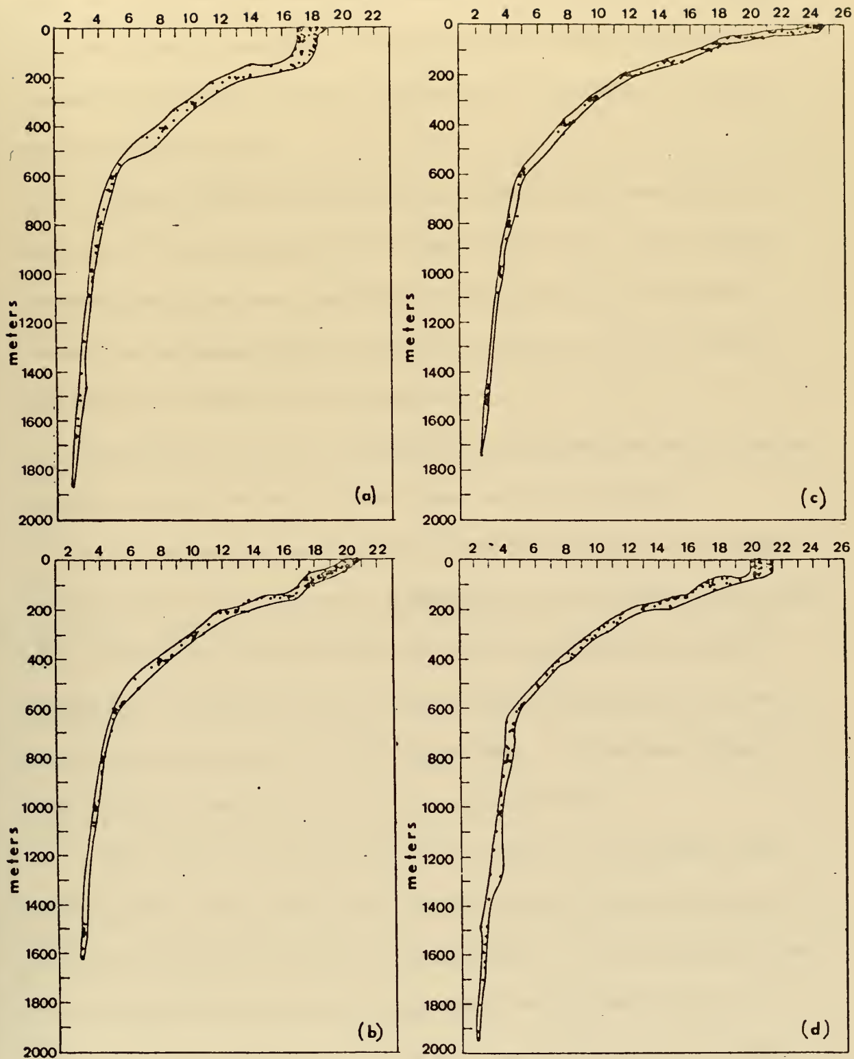
Figure 6. Seasonal Vertical Temperature Profiles at OWS November, (a) Late Winter (2-19 May, 1967), (b) Summer-to-Winter (15 Jun-1 Jul, 1967), (c) Summer (3-24 Sep, 1967), and (d) Summer-to-Winter (26 Nov-17 Dec, 1967). (after Husby, 1969).
