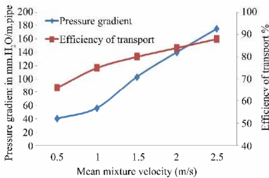
Figure 3. Variation of slurry performance characteristics for sand slurry with solid concentration 1% by volume and particle diameter d_s = 0.25 mm. versus mean mixture velocity.
