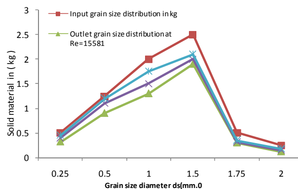
Figure 19. Effect of Reynolds number's on grain size distribution at pipe outlet at total input concentration of 0.119% by volume of iron oxide.
