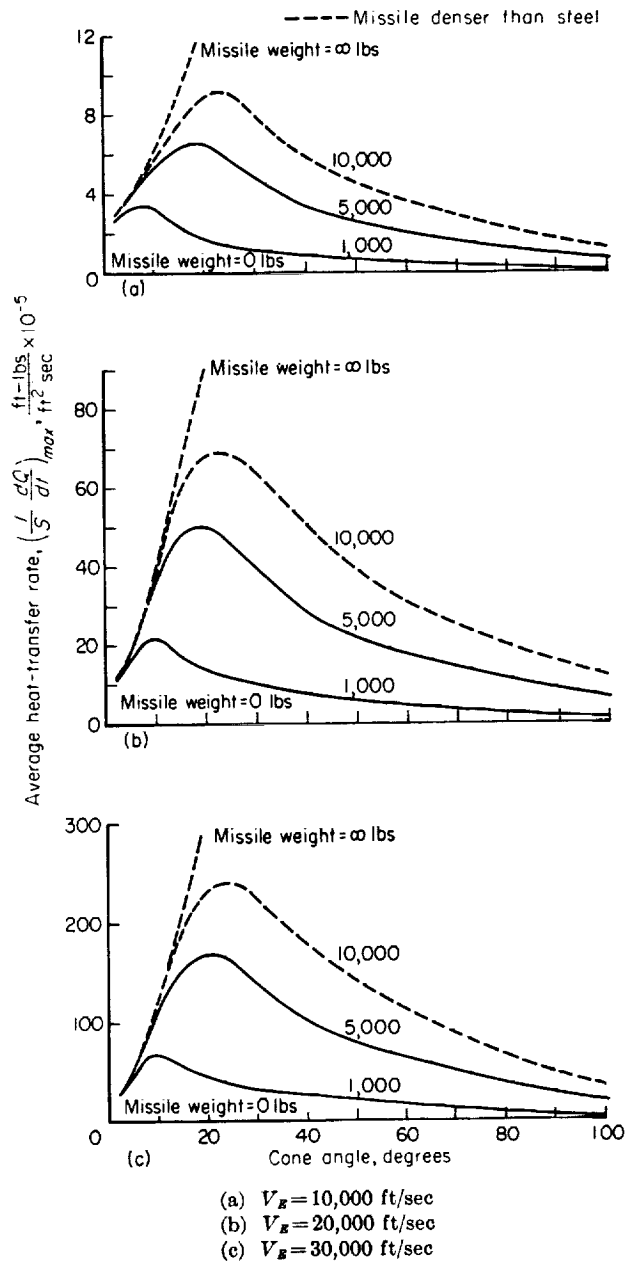
FIGURE 8.—Maximum average rate of convective heat transfer to conical missiles of the same volume entering the earth's atmosphere at an angle of 30° to the horizontal and velocities of 10,000, 20,000, and 30,000 ft/sec (volume = 16.34 cu ft).
