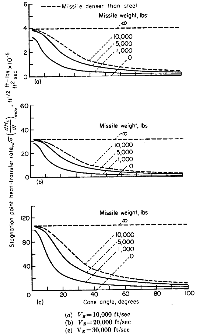
FIGURE 11.—Maximum rate of convective heat transfer to the stagnation point of spherically tipped cones of the same volume entering the earth's atmosphere at an angle of 30^\circ to the horizontal and velocities of 10,000, 20,000, and 30,000 ft/sec (volume = 16.34 cu ft).
