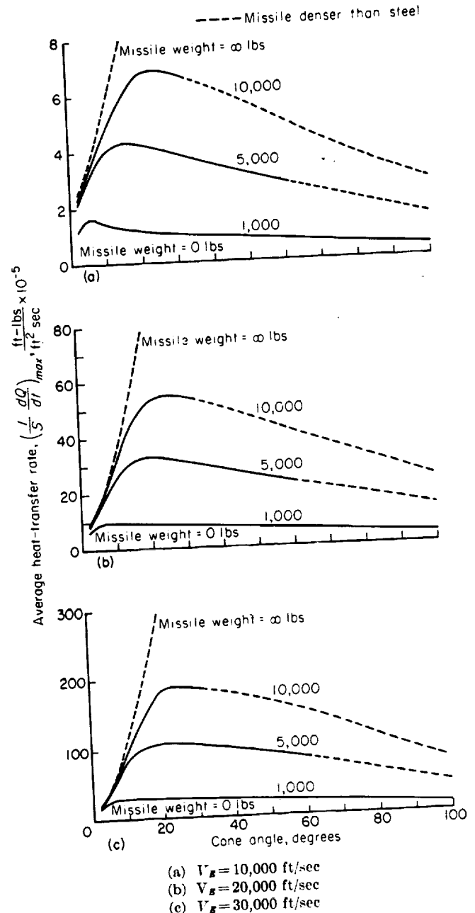
FIGURE 7.—Maximum average rate of convective heat transfer to conical missiles of the same base area entering the earth's atmosphere at an angle of 30^\circ to the horizontal and velocities of 10,000, 20,000, and 30,000 ft/sec (base area = 10 sq ft).
