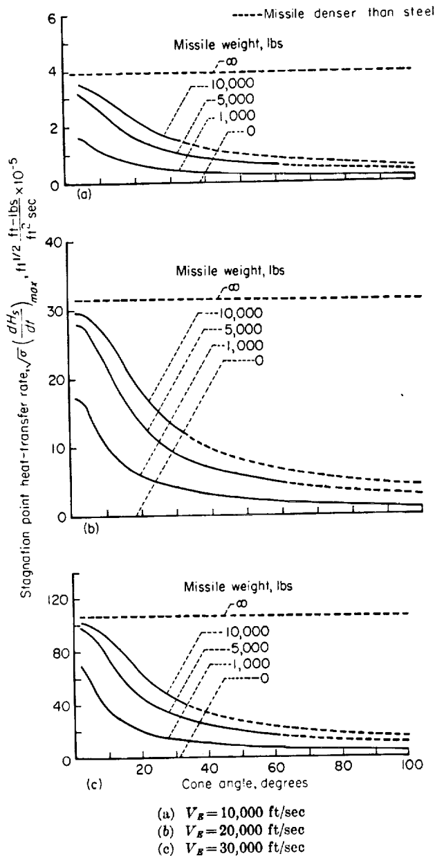
FIGURE 10.—Maximum rate of convective heat transfer to the stagnation point of spherically tipped cones of the same base area entering the earth's atmosphere at an angle of 30^\circ to the horizontal and velocities of 10,000, 20,000, and 30,000 ft/sec (base area = 10 sq ft).
