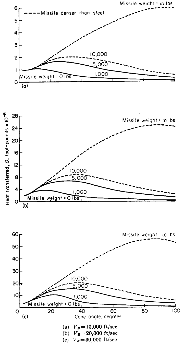
FIGURE 6.—Convective heat transferred at impact to conical missiles of same volume entering the earth's atmosphere at an angle of 30^\circ to the horizontal and velocities of 10,000, 20,000, and 30,000 ft/sec (volume = 16.34 cu ft).
