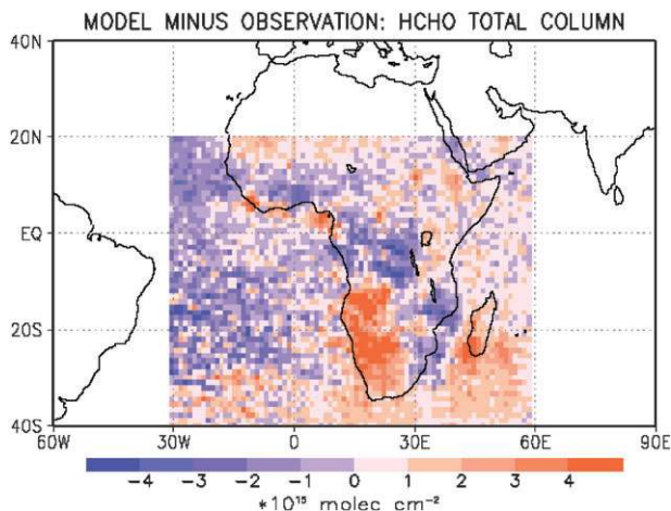
Fig. 10 The difference (\text{TC}(\text{HCHO})_{\text{model}} - \text{TC}(\text{HCHO})_{\text{GOME}}) in units of 1 \times 10^{15} molecule \text{cm}^{-2} between modeled total HCHO columns and HCHO columns, retrieved from GOME measurements.
