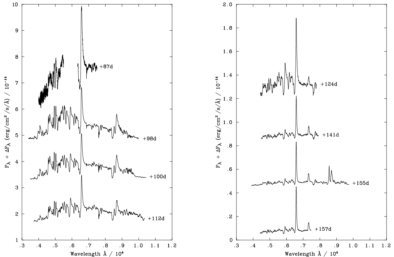
Figure 2. Spectral evolution of SN 2003gd from 87–157 d after explosion, where the spectra have been arbitrarily shifted in flux for clarity.
