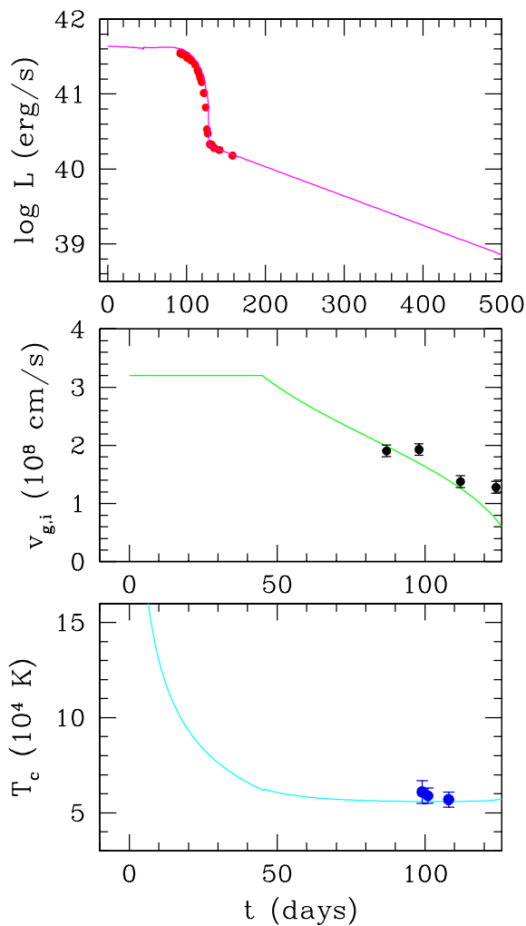
Figure 18. Results for model A showing V-band luminosity, L , velocity of metal ( \text{Sc II } \lambda \text{ 6246} ) lines, v_{g,i} , and continuum temperature, T_c , as a function of time for SN 2003gd. The adopted distance modulus and the estimated total reddening are \mu = 29.32 and A_V = 0.42 . The assumed explosion date is JD 245 2717. The solid lines represent the curves from the semi-analytic model of Zampieri et al. (2003).
