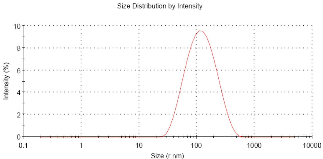
Fig.2 Size distribution of particle conglomerate of water+0.05wt% \text{CeO}_2 +1wt% surfactant (Sorbitan monostearate).
