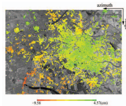
Fig.1 The linear velocity map of Tianjin area from the primary PS-like method
