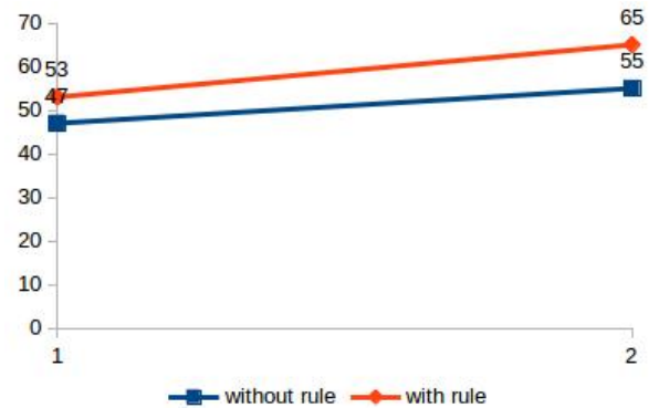
Figure 2: Accuracy Graph
