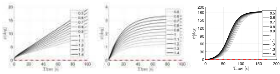
Fig. 22: Evolution of the attitude of the object with one leader in a group of ground agents. f_{\text{int}} = 0 in the first column, f_{\text{int}} > 0 in the second column, and f_{\text{int}} < 0 in the third column. The external disturbance torque \tau_{e,z} is applied. We recall that its intensity m_{ext} , is expressed in the legend in Nm.
