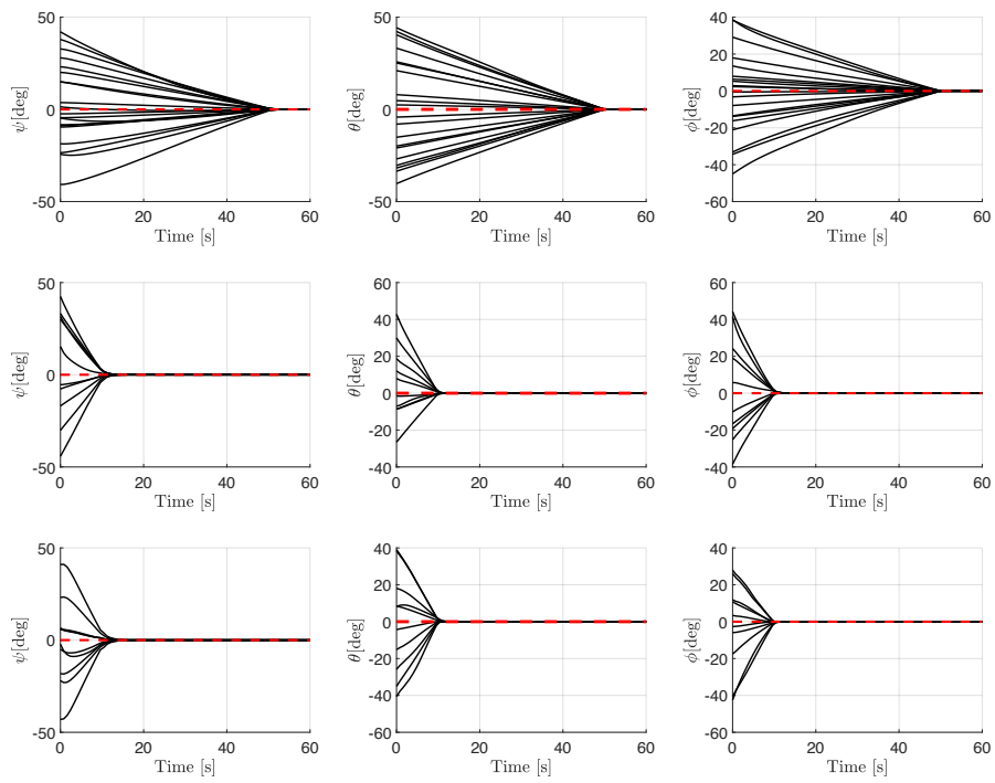
Fig. 18: Evolution of the attitude of the object with three leaders in a group of floating agents. f_{int} = 0 in the first row, f_{int} > 0 in the second row, and f_{int} < 0 in the third row. Notice that, even though the attitude converges to the desired value in each case, the presence of non-zero internal forces increases the convergence rate.
