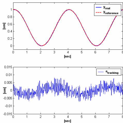
Fig. 5. Closed-Loop control with disturbance compensation
