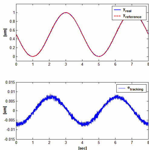
Fig. 7. Sinusoidal reference tracking with PID and disturbance compensation
