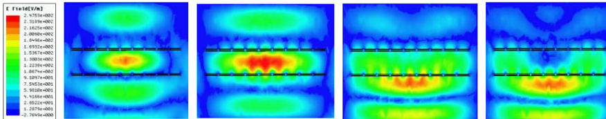
Figure 3b. E -field distribution in free space with metamaterial structure.
