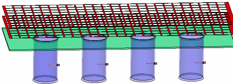
Figure 7a. Model of the 1 \times 4 antenna array.
