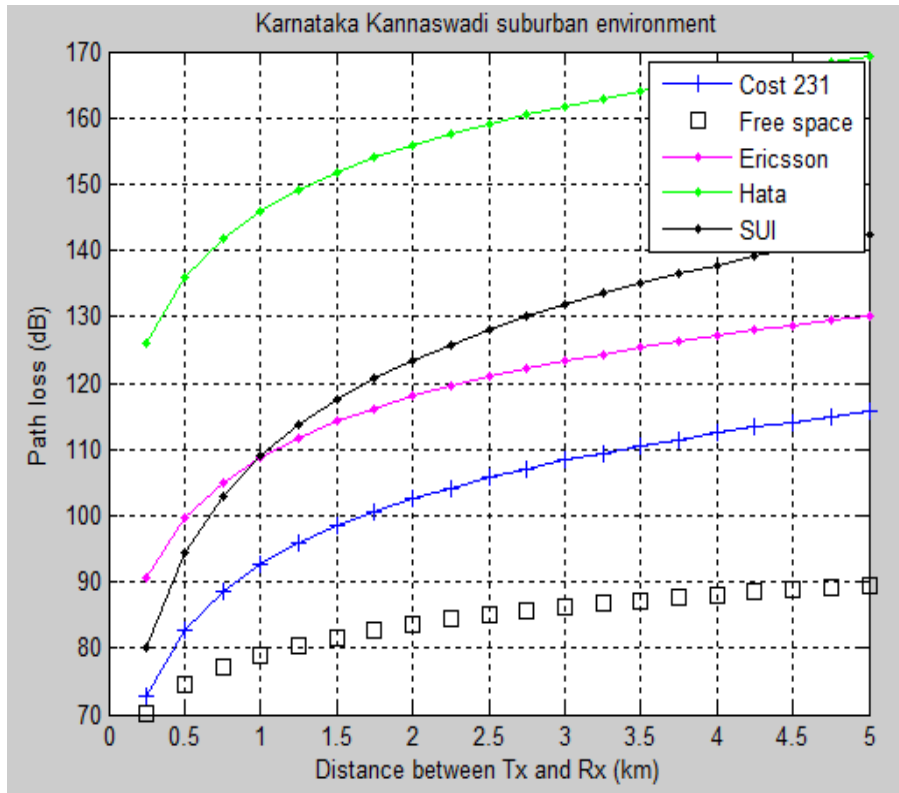
Figure 8.c. . Path loss at Kannaswadi suburban at 940 MHz GSM frequency
