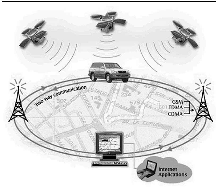
Figure 4.1.a. Measurement framework
