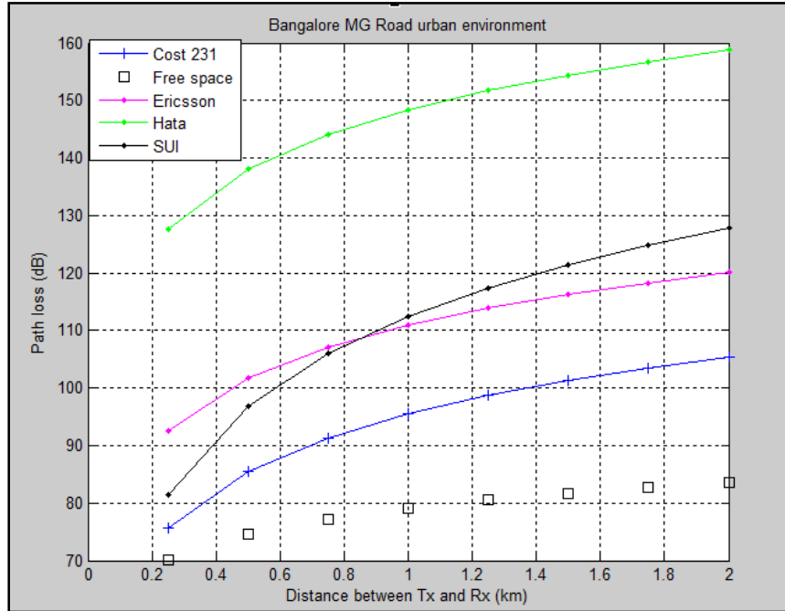
Figure 8.a. Path loss at MG road urban at 940 MHz GSM frequency
