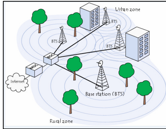
Figure 1.a. GSM framework
