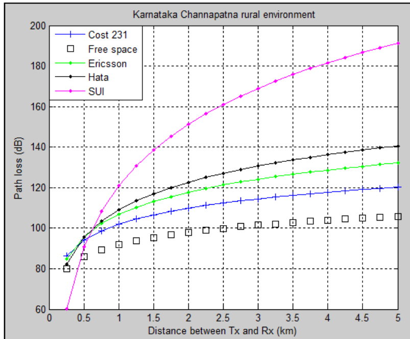
Figure 8.b. Path loss at Channapatna rural at 940 MHz GSM frequency
