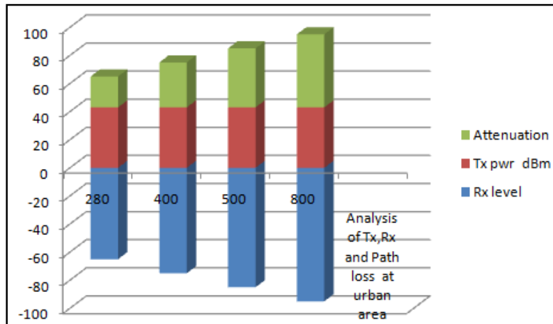
Figure 9.a Analysis of path loss at urban area
