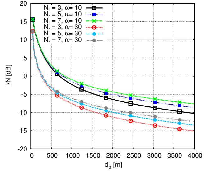
Fig. 5. Aggregate interference in the omnidirectional worst-case scenario
