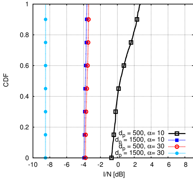
Fig. 6. Aggregate interference CDF with omnidirectional BSs
