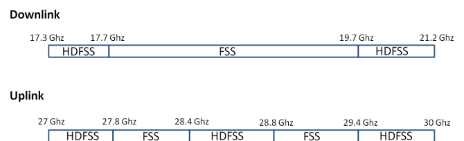
Fig. 1. FSSs and HDFSSs spectrum allocation
