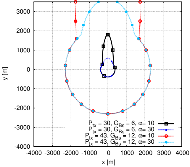
Fig. 4. -10 dB region with a single interferer
