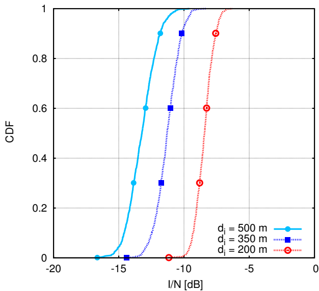
Fig. 10. Aggregate interference CDF considering different BSs intersite distances
