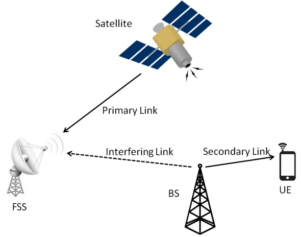
Fig. 2. FSS-BS coexistence scenario
