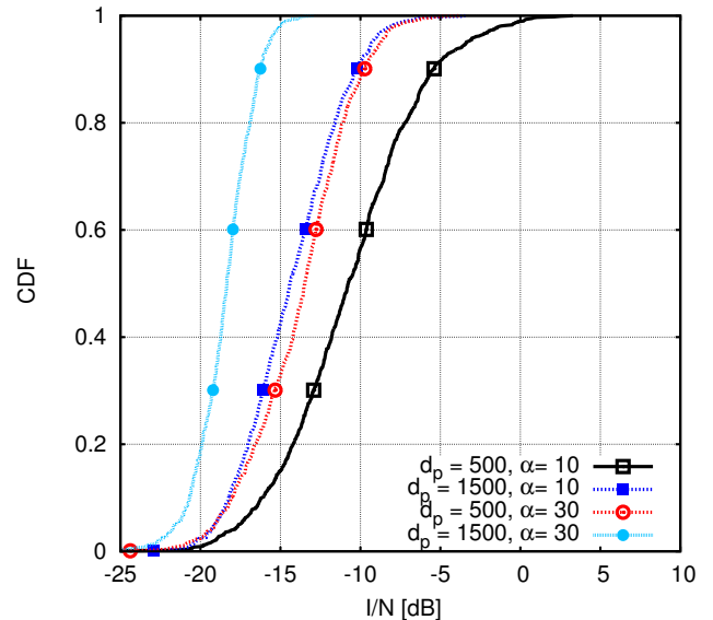
Fig. 9. Aggregate interference CDF considering BSs with N_a = 64
