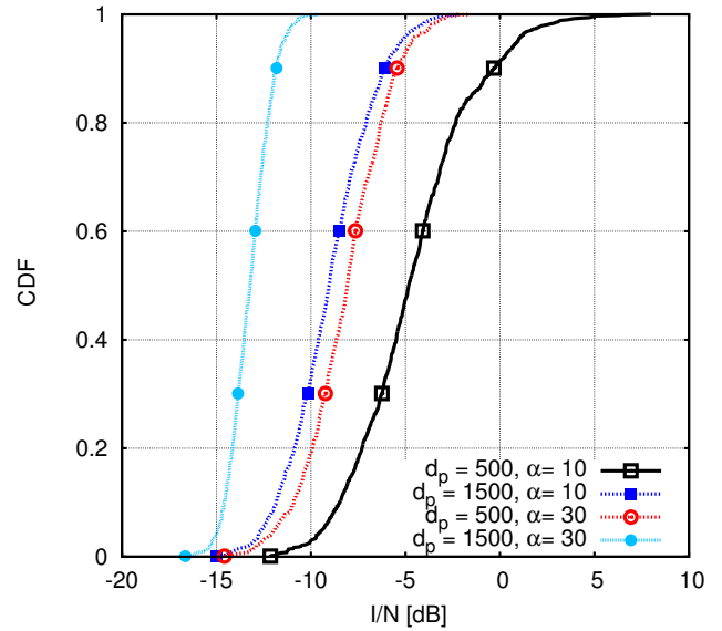
Fig. 8. Aggregate interference CDF considering BSs with N_a = 16
