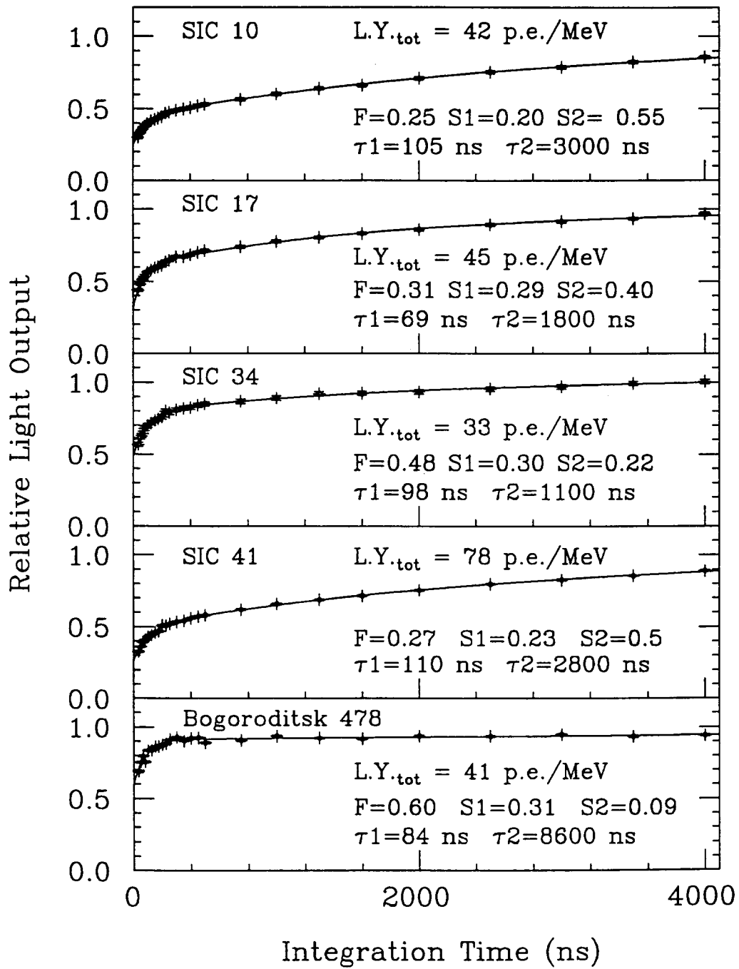
Figure 12: Light yield of five small size PbWO 4 samples as a function of integration time.
