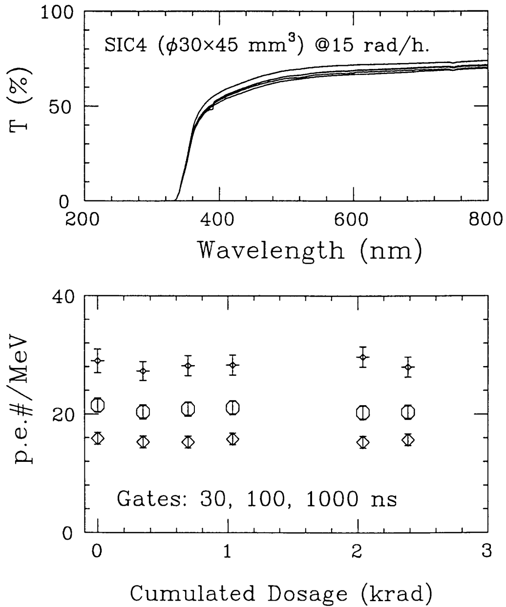
Figure 22: Top: the longitudinal transmittance as a function of wavelength before and after irradiation for sample 4 from SIC (4.5 cm long). Bottom: the light yield integrated in 30, 100 and 1000 ns is shown as a function of cumulative dose.
