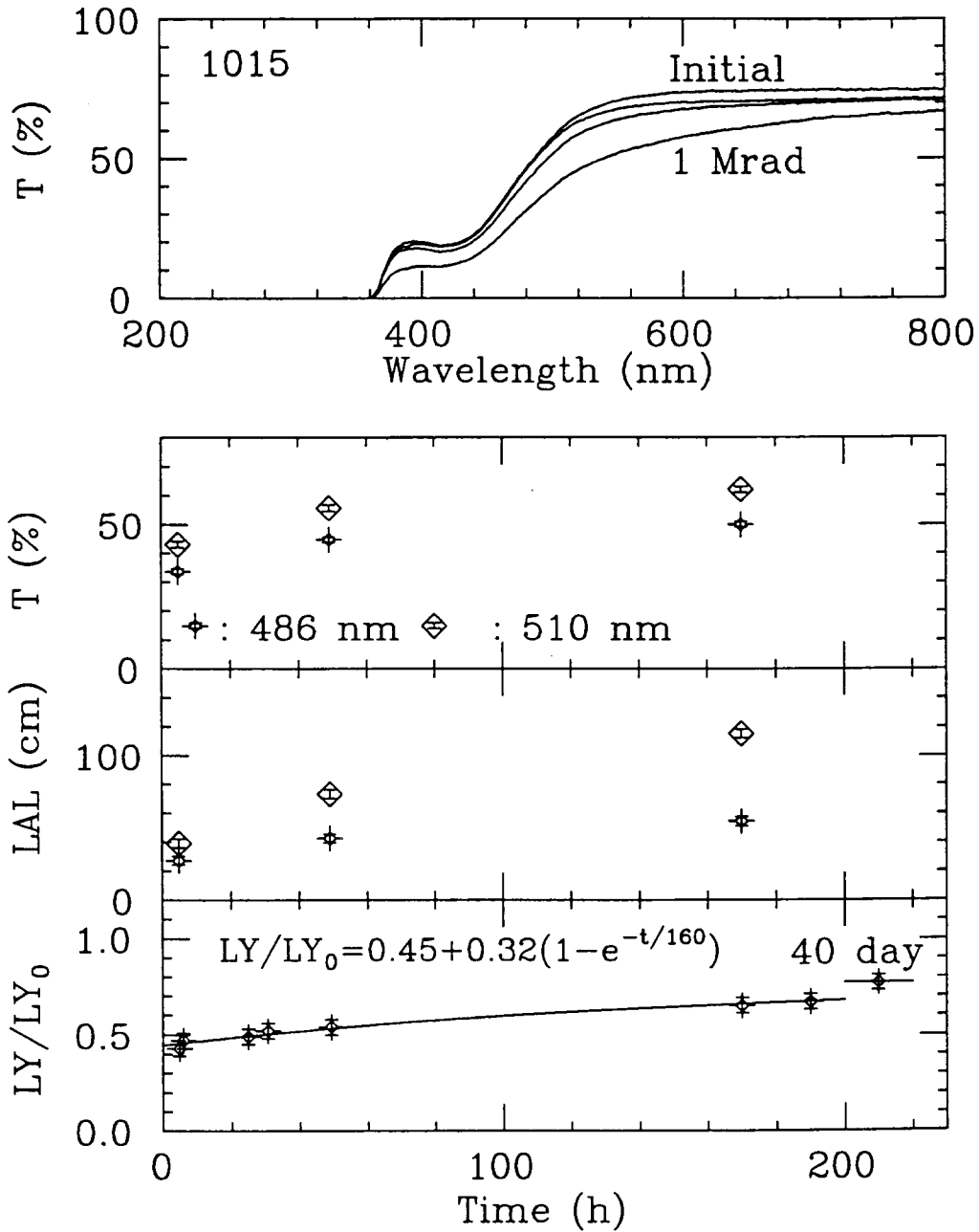
Figure 19: Recovery from radiation at room temperature for sample 1015. The curves are, from top to bottom: before irradiation, 170, 49 and 4.8h after 1 Mrad irradiation. Bottom figures show the recovery in transmittance, light attenuation length and light yield with time. The rightmost data point was taken after 40 days after 1 Mrad irradiation.
