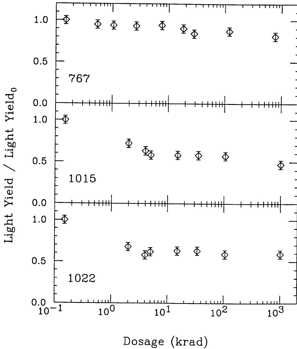
Figure 18: The light output normalized to the value before irradiation as a function of cumulative dose for crystals 767, 1015 and 1022. The actual doses are the same as in Figure 16.
