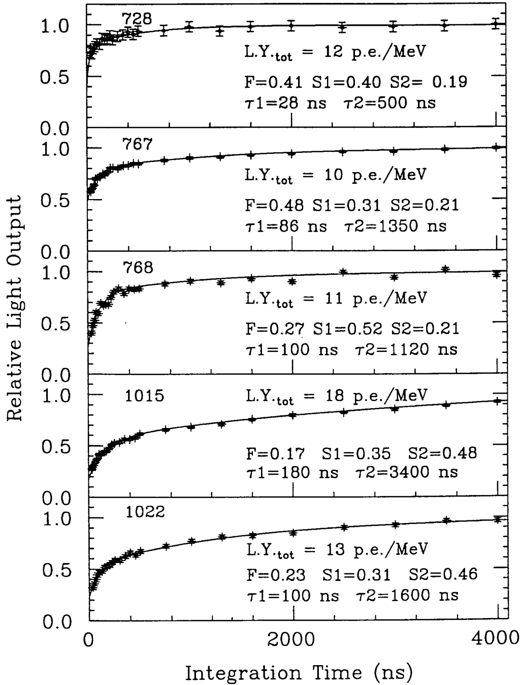
Figure 11: Light yield of five full size PbWO 4 samples is shown as a function of integration time.
