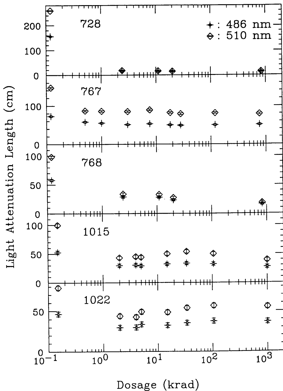
Figure 17: The light attenuation length at 486 and 510 nm as a function of cumulative dose for crystals 728, 767, 768, 1015 and 1022. The actual doses are the same as in Figure 16.
