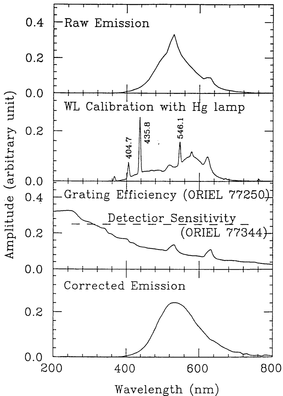
Figure 2: Corrections to the emission data. From top to bottom: typical uncorrected data of a measured emission spectrum; wavelength calibration with a Hg lamp; measured grating efficiency (solid) and the detector sensitivity (dashed line); the emission spectrum after corrections.
