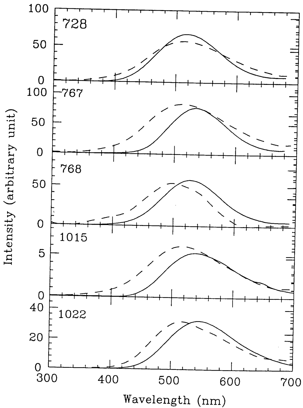
Figure 7: Photo- (solid) and radio- (dashes) luminescence of five full size PbWO 4 samples as a function of the wavelength.
