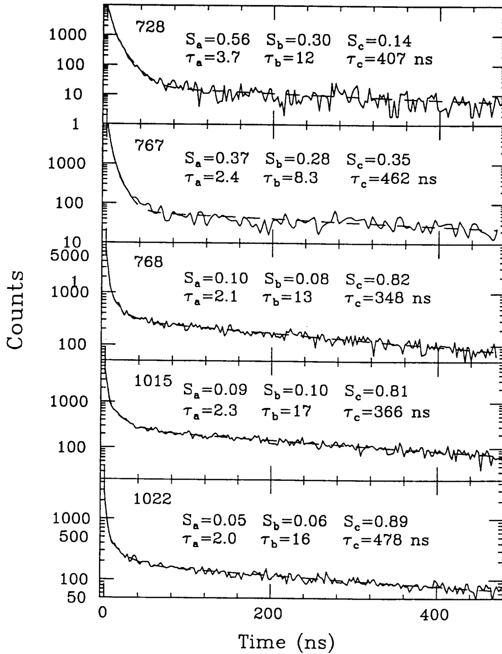
Figure 13: Decay time spectra measured with the single photon counting method for five full size samples.
