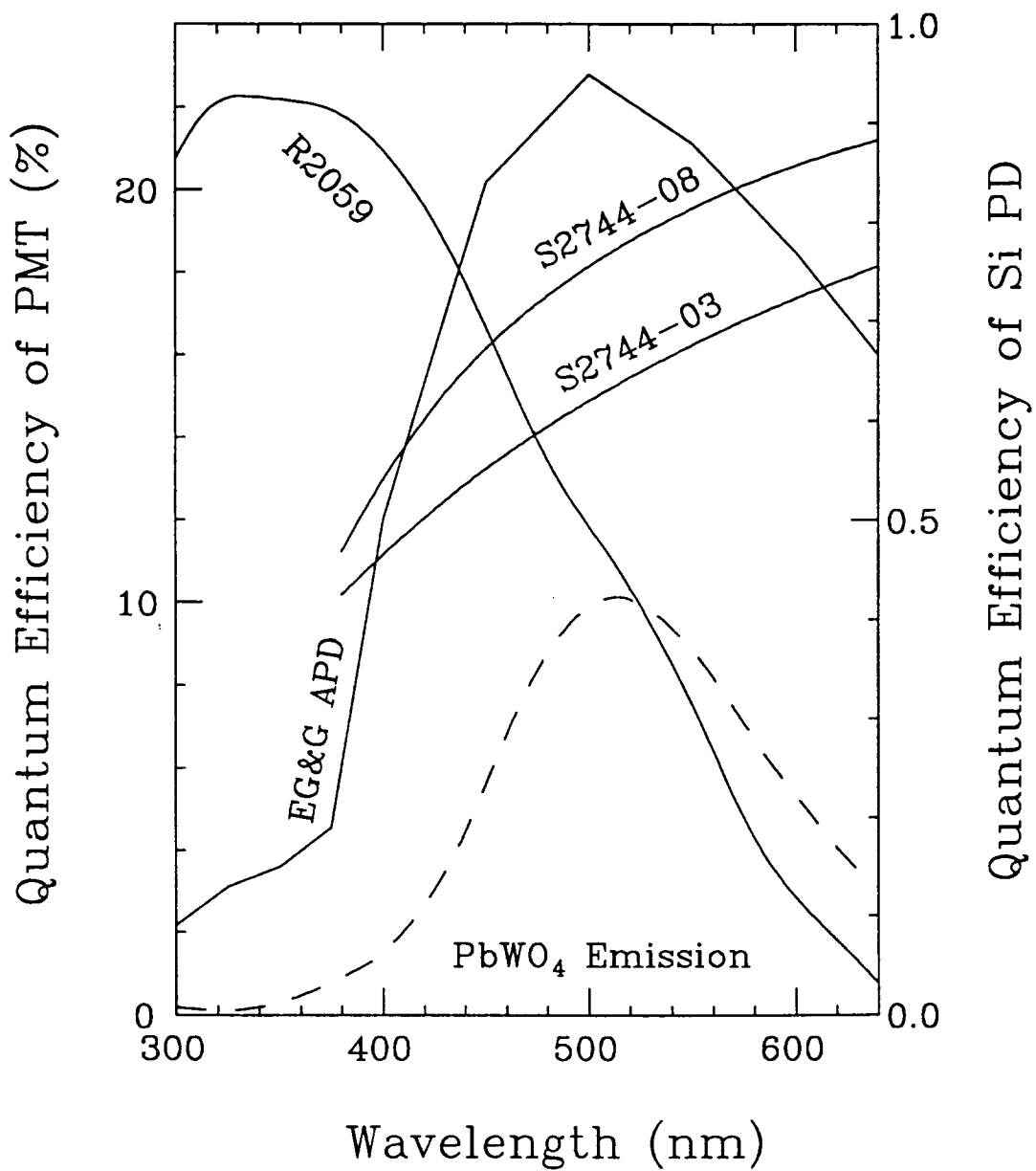
Figure 9: PbWO 4 emission and quantum efficiency of various photodetectors.
