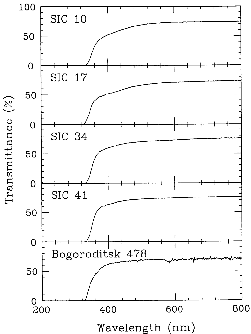
Figure 6: Transmittance of five small size PbWO 4 samples as a function of wavelength. The light path is along the longest edge of the sample.
