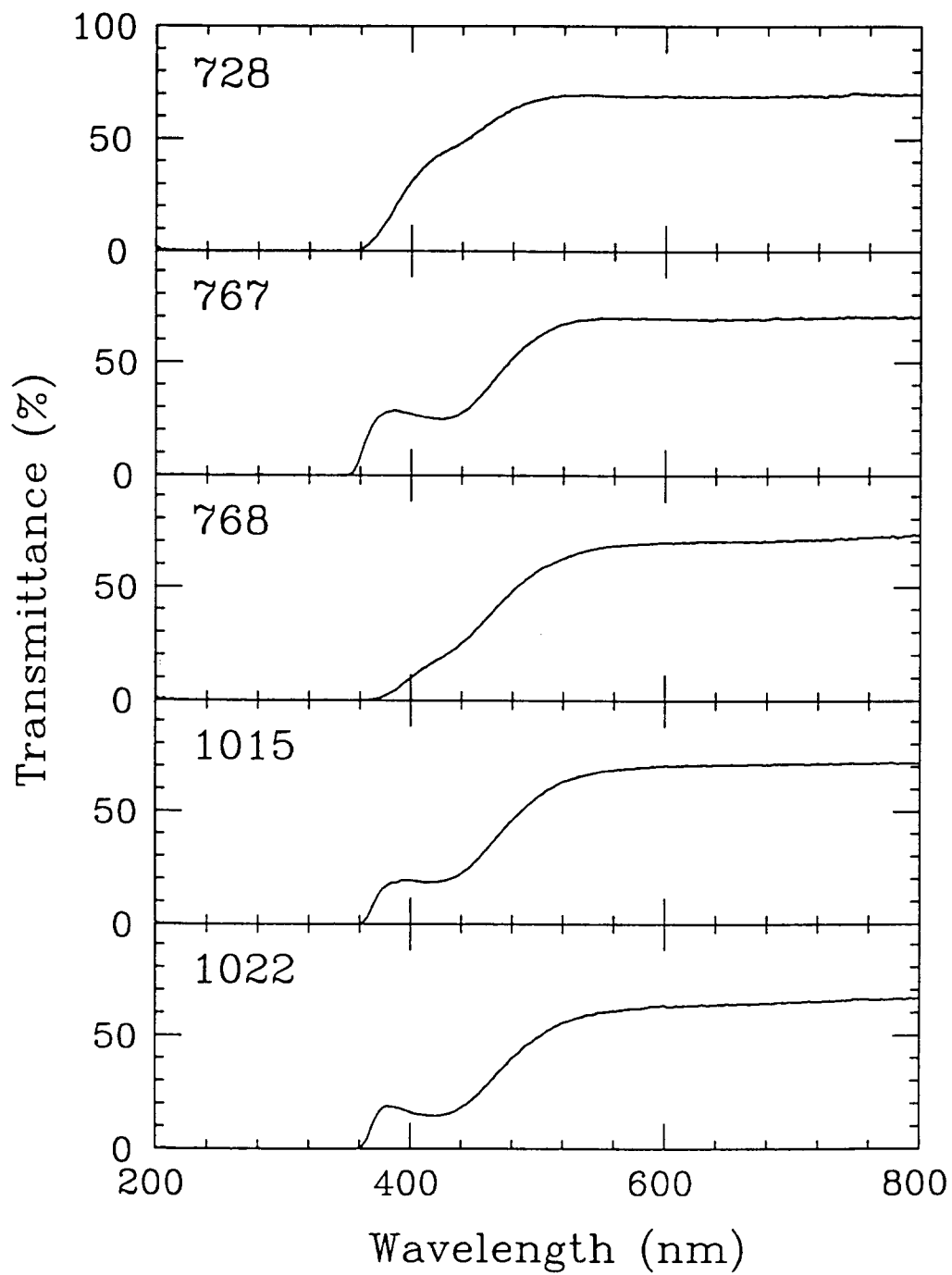
Figure 5: Longitudinal transmittance of five 21.3 cm PbWO 4 samples as a function of the wavelength.
