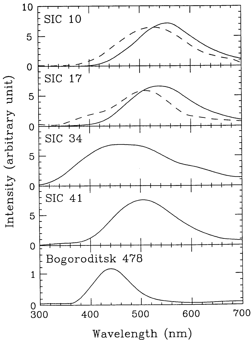
Figure 8: Photo- (solid) and radio- (dashes) luminescence of five small \text{PbWO}_4 samples as a function of the wavelength.
