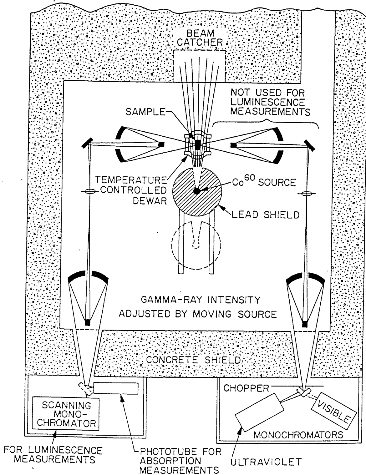
Figure 4: The layout of the Gamma Ray Irradiation Facility at Brookhaven National Laboratory.
