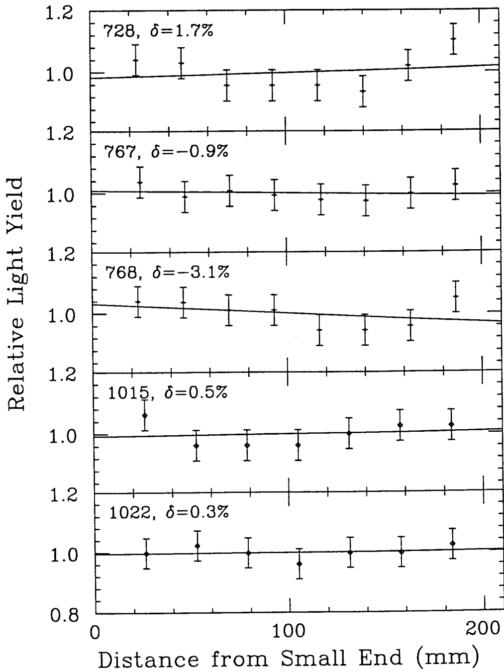
Figure 10: Light response uniformity of five full size PbWO 4 samples is shown as a function of the distance to the small end of the crystal.
