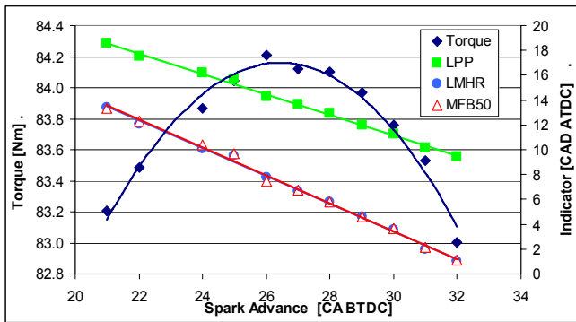
Fig. 2 Engine torque and combustion phase indicators as functions of spark advance (2500 rpm, MAP=100 kPa, \lambda=1.0 , Fuel: Natural Gas)
