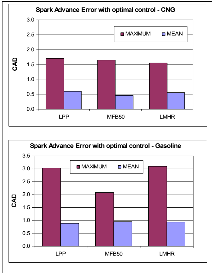
Fig. 3 Spark advance errors related to the indicators mean set point (Top: CNG, Bottom: Gasoline)
