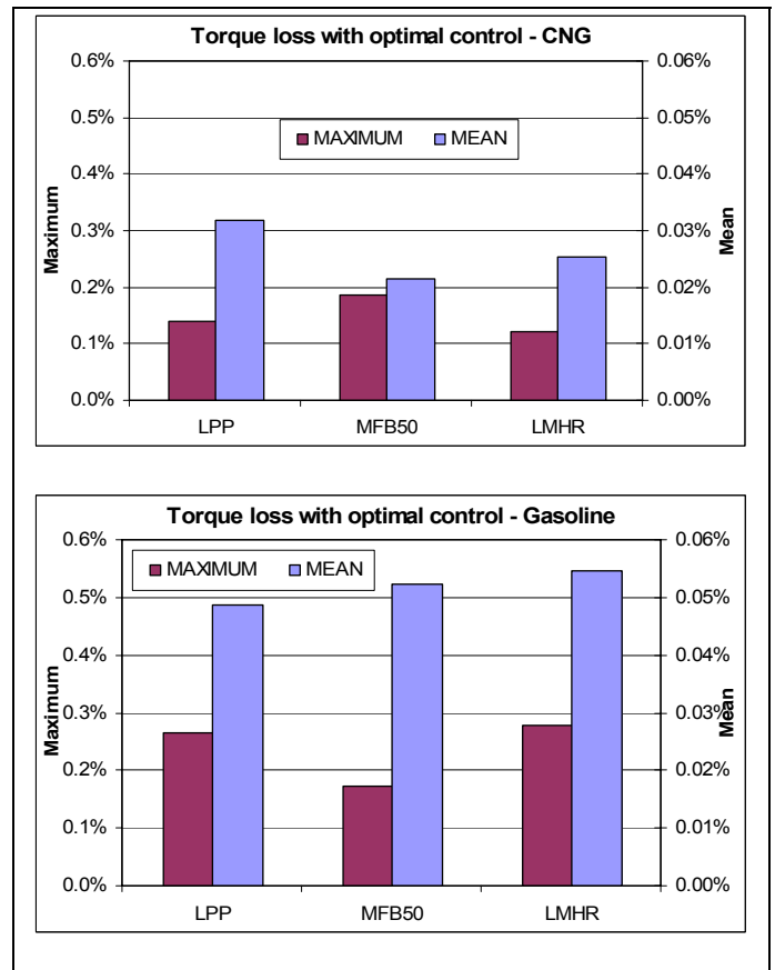
Fig. 4 Torque losses related to the indicators mean set point (Top: CNG, Bottom: Gasoline)
