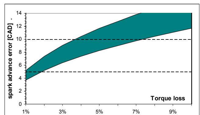
Fig. 1 Torque loss due to bad spark timing control
