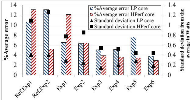
Fig. 2. Average error and standard deviation for all expressions.
