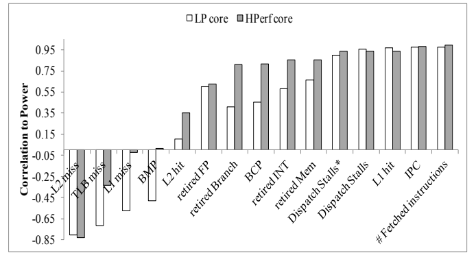
Fig. 1. Correlation of various performance counters to power consumed.
