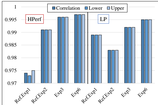
Fig. 4. The correlation and upper and lower levels of the confidence interval for a confidence level of 99%. Results are shown for selected expressions obtained for the HPerf and LP cores.
