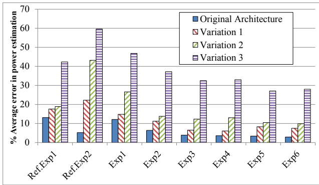
Fig. 6. Average error between estimated and calculated power (using Watch) when the expression derived for the HPerf core is used to estimate power on a variation of that architecture. Variation 1, 2 and 3 are defined in Table III. other, if the right counters are chosen. The power expression obtained for one architecture can thus be used as a first order estimate for the power on a small variation of that architecture.
