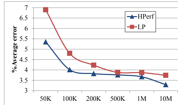
Fig. 7. Error as a function of interval length for the HPerf and LP cores.
