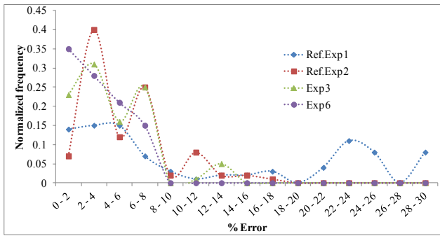
Fig. 3. Normalized frequency distribution of the error of selected expressions for the HPerf core. Points connected by dotted lines to show the trend.
