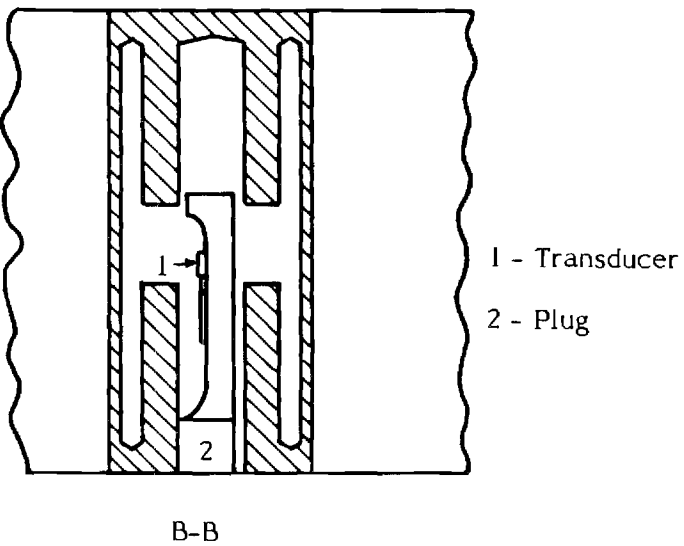
(b) Cross-sections
