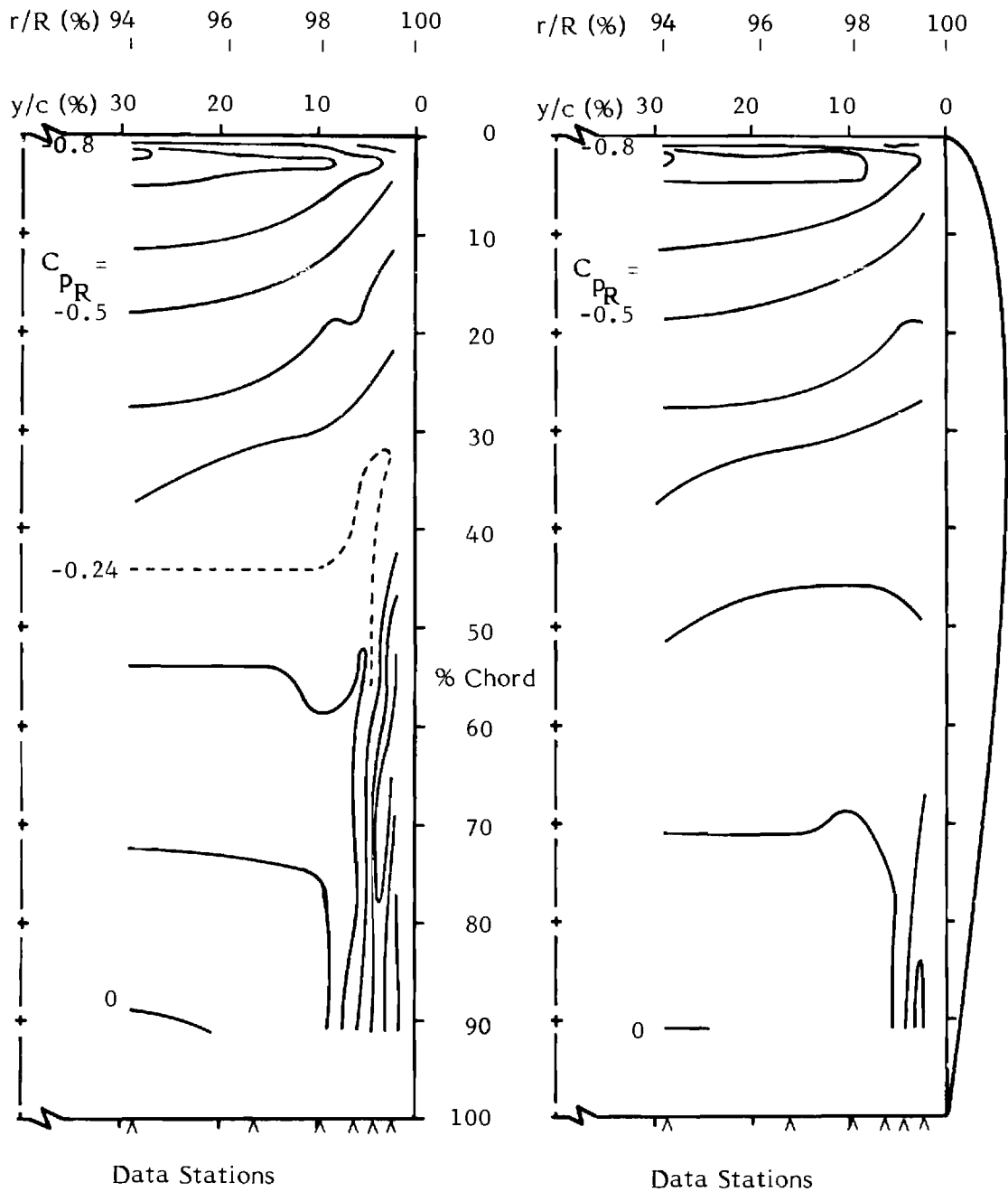
(b) Upper surface, flat tip
