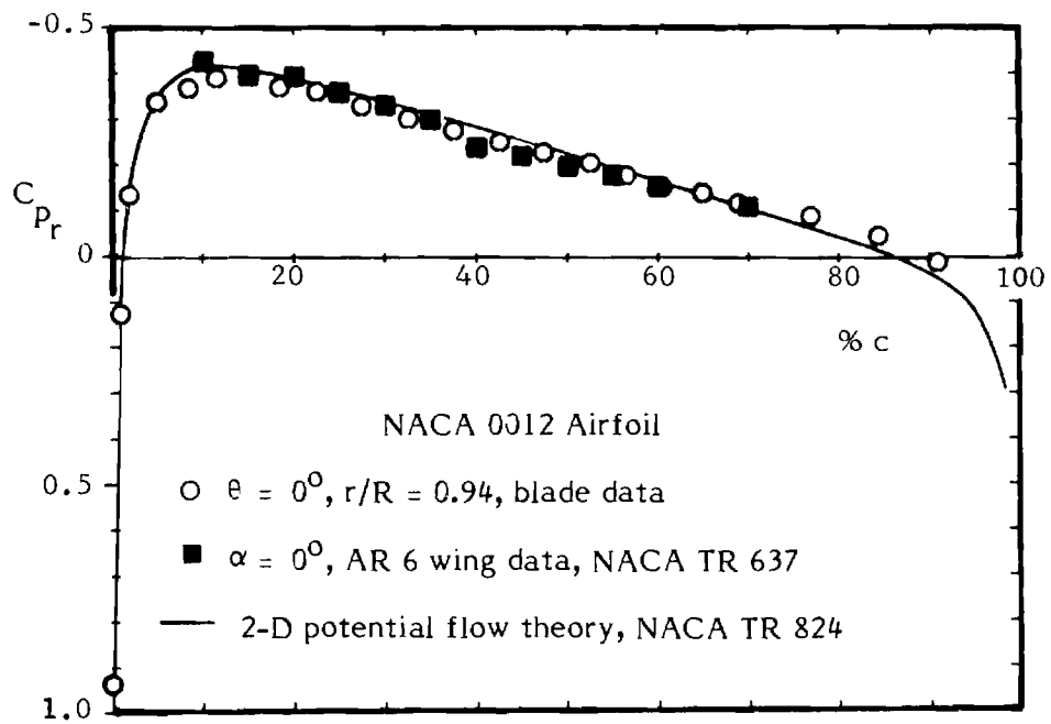
Figure 4. - Chordwise pressure coefficient data measured on a rotating blade compared with measured data on a wing of aspect ratio 6 and with two-dimensional potential flow theory results.
