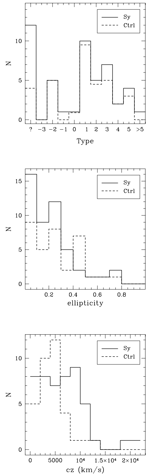
FIG. 2.—Distribution of Seyfert and control sample before removing the galaxies for which no reliable bar classification could be made.
