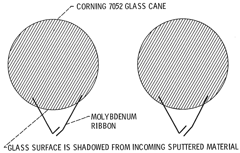
Figure 16. - Cross section of shadow shielded vector grid concept.
