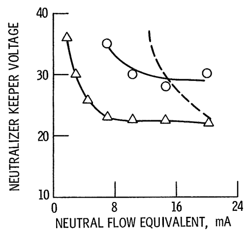
Figure 6. - Keeper discharge characteristics of neutralizers.
