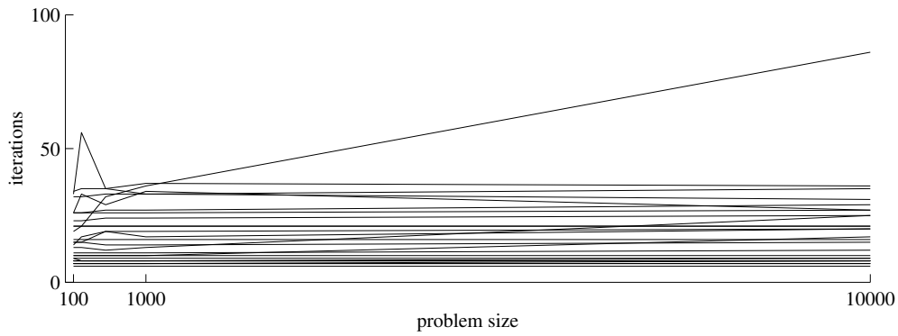
FIG. 7. STIR performance with exact Newton steps
