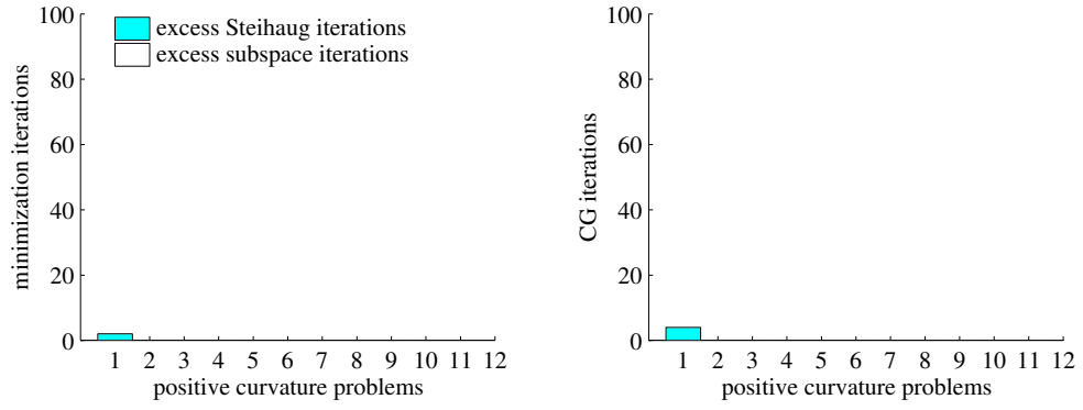
FIG. 3. Comparison of subspace and Steihaug trust region methods for unconstrained problems
