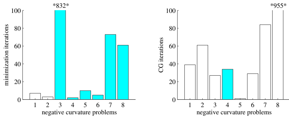
FIG. 4. Comparison of subspace and Steihaug trust region methods for unconstrained problems
