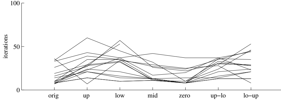
FIG. 10. STIR method with inexact Newton steps at varied starting points
