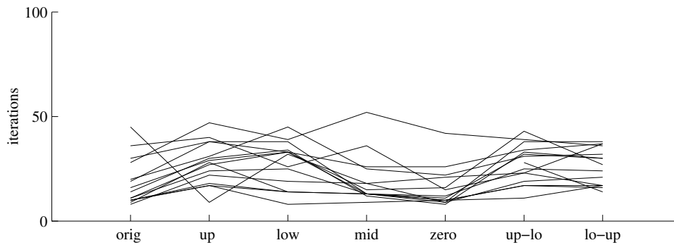
FIG. 9. STIR method with exact Newton steps at varied starting points
