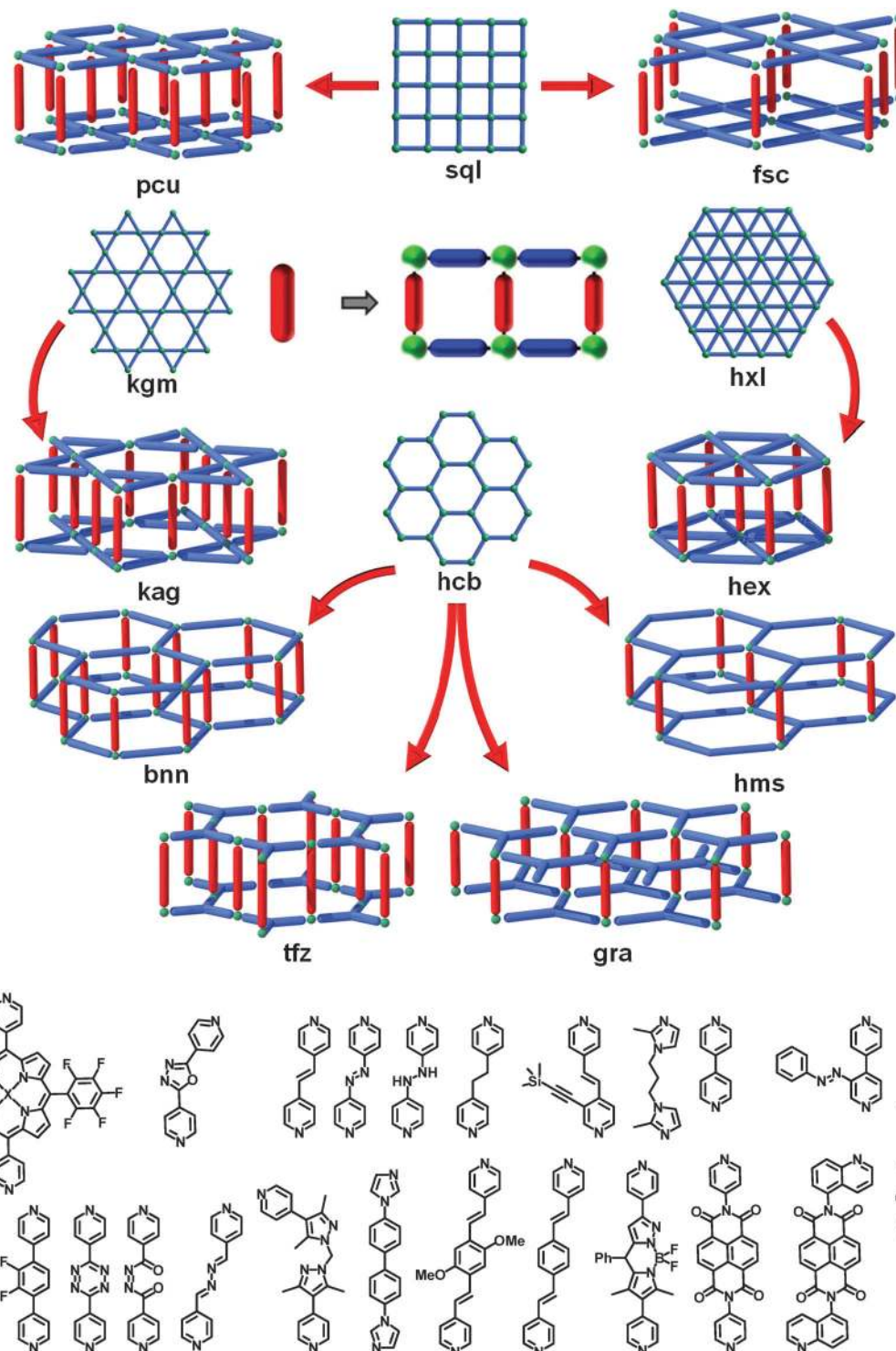
Fig. 28 Schematic of the A–A pillaring of sql , kgm , hxl , and hcb layers to form the pcu , fsc , kag , hex , bnn , hms , gra , and tfz nets (top), and a non-exhaustive list of ligands that have been used for this type of pillaring (bottom).
