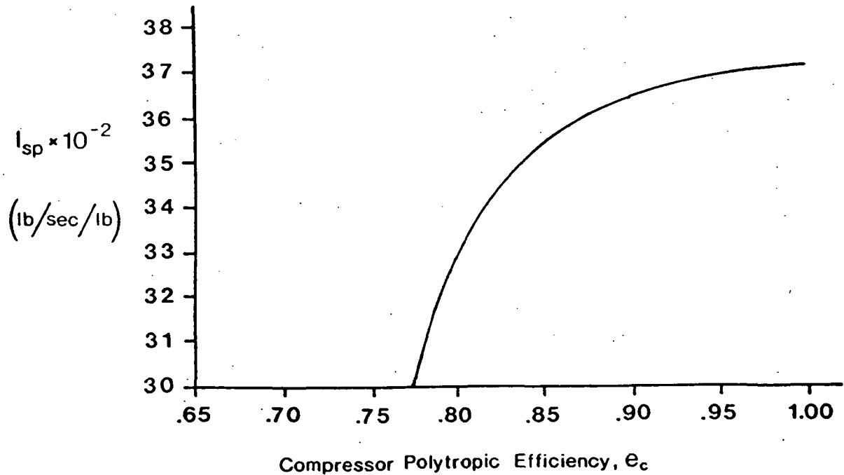
Figure 2.8 Effect of Core Compressor Polytopic Efficiency on Specific Impulse at Mach 2.7 Cruise
