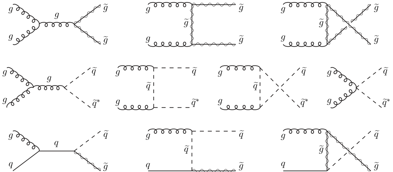
Figure 10.2: Feynman diagrams for gluino and squark production at hadron colliders from gluon-gluon and gluon-quark fusion.
