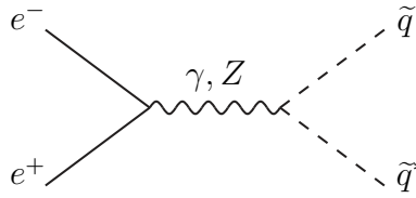
Figure 10.10: Diagram for squark production at e^+e^- colliders.
