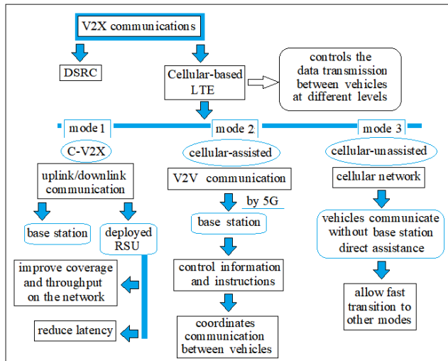
FIGURE 13. V2X modes.
