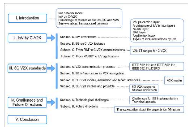
FIGURE 4. Paper's structure.
