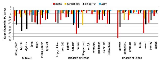
FIGURE 14. Percentage change in IPC values for reduced pipeline width for 64-bit binaries.
