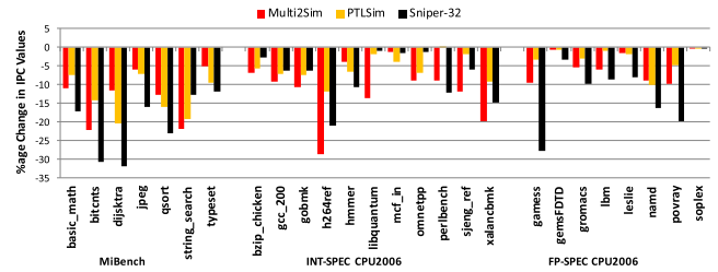
FIGURE 13. Percentage change in IPC values for reduced pipeline width for 32-bit binaries.
