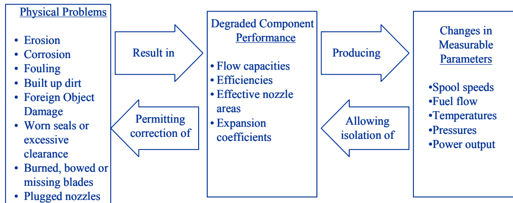
Figure 9.—Diagram indicating information flow for turbine engine gas path diagnostics.
