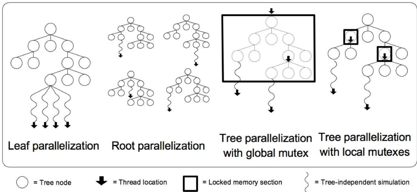
Fig. 8. Parallelisation approaches for MCTS [59].
