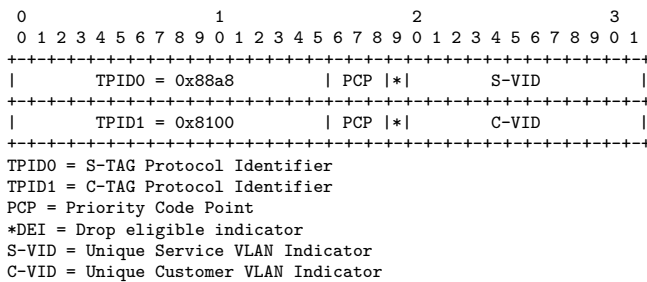
Figure 19: 802.1ad header
