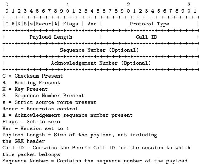
Figure 6: PPTP Header
