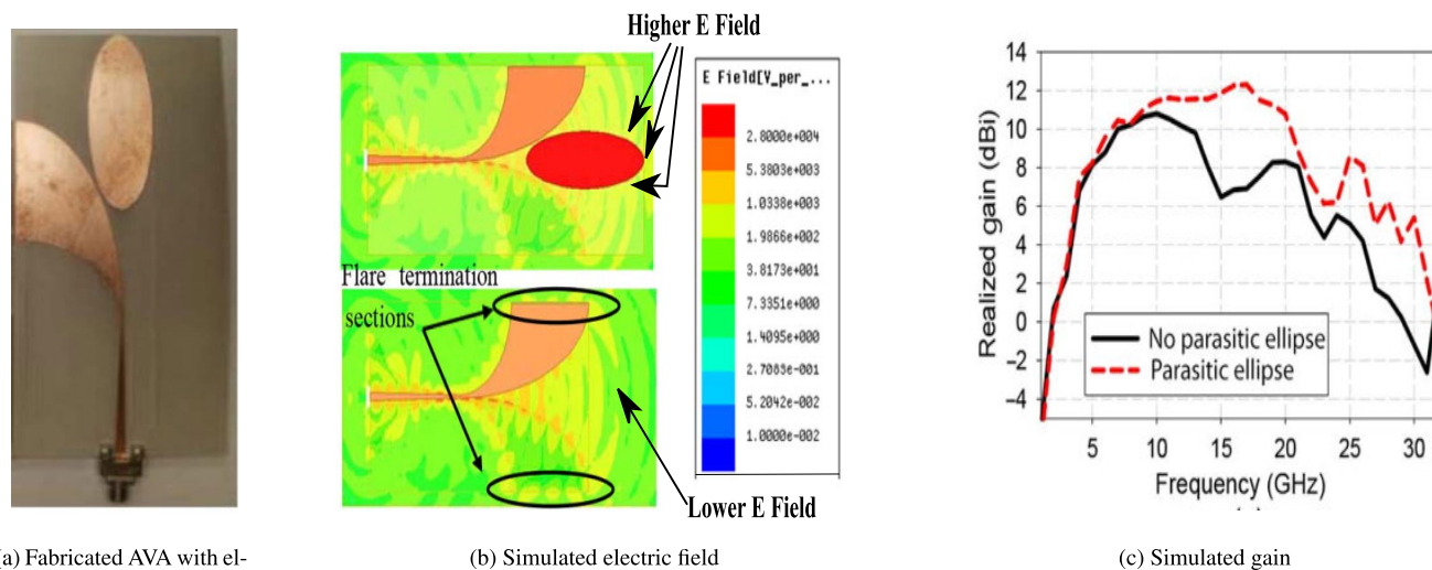
FIGURE 13. Effect of parasitic patch [42].
