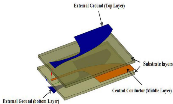
FIGURE 16. Structure of balanced antipodal Vivaldi antenna (BAVA) [68].
