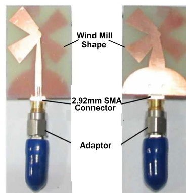
(a) Fabricated windmill shaped AVA
