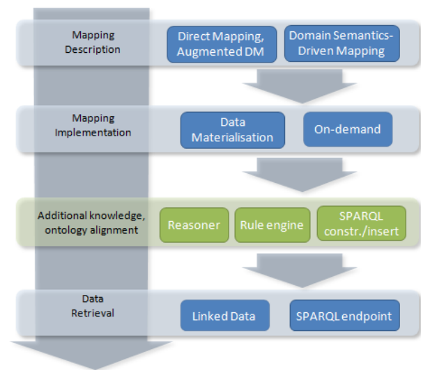
Fig. 2. Semantic enrichment. The green layer depicts strategies aimed at a posteriori production of additional semantic data
