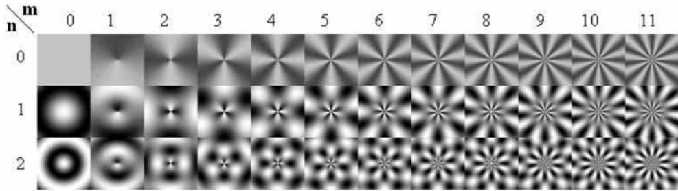
Fig. 36. Real parts of the ART basis functions
