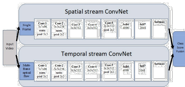
Figure 8. Two-stream architecture with the spatial stream using images and the temporal stream using optical flows. Source: [102].
