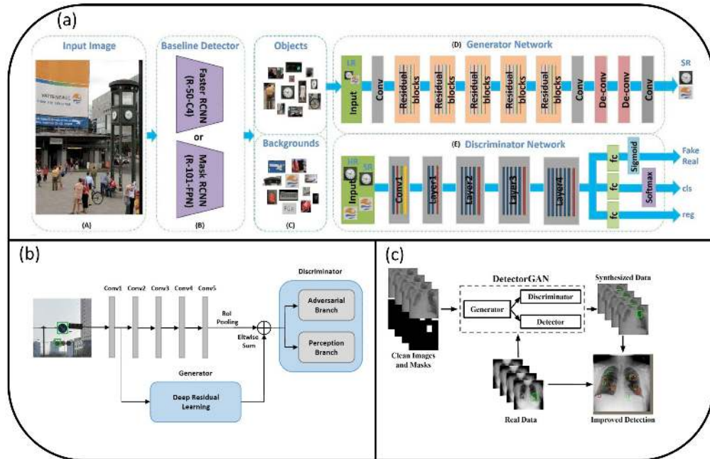
Figure 27: Architecture diagram of (a) SOD-MTGAN [208] (b) Perceptual GAN [203] and (c) Detector GAN [204].
