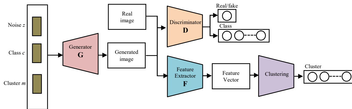
Figure 12: Architecture diagram of clustering based GAN for solving intra-class imbalance presented by N. Hase et al. [155]
