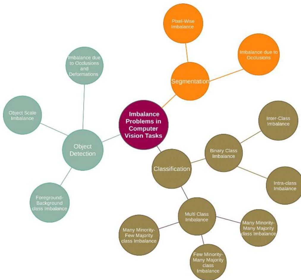
Figure 2: Proposed taxonomy for the review of imbalanced problem in computer vision tasks
