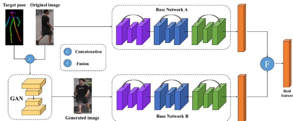
Figure 17: Architecture diagram of pose-normalized GAN presented by Qian et al. [170]
