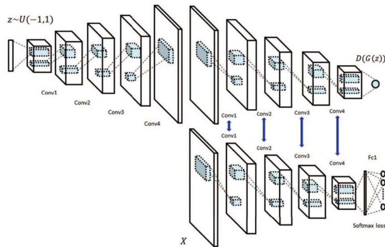
Figure 20: Complete fine-grained Plankton classifier architecture used by C. Wang et al. [182]
