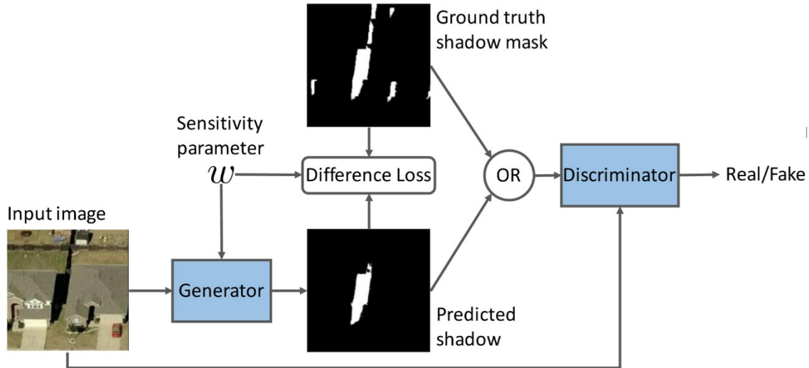
Figure 32: Illustration of Sensitivity conditional GAN[218]
