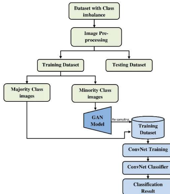
Figure 11: flowchart of GAN-based oversampling technique
