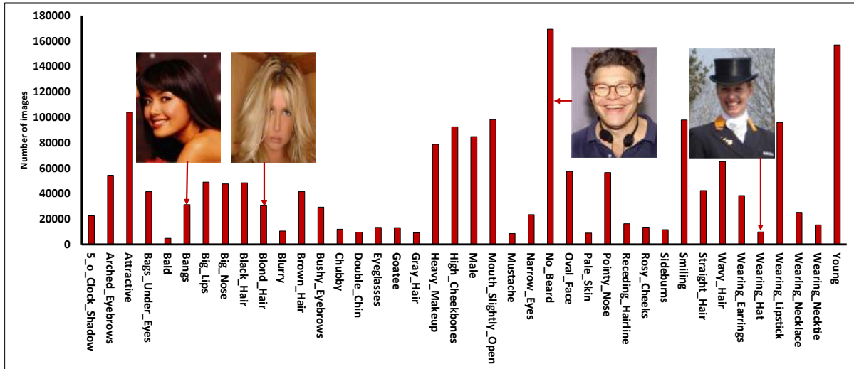
Figure 13: Imbalanced distribution of 40 binary face attributes (positive and negative) on CelebA dataset [161]
