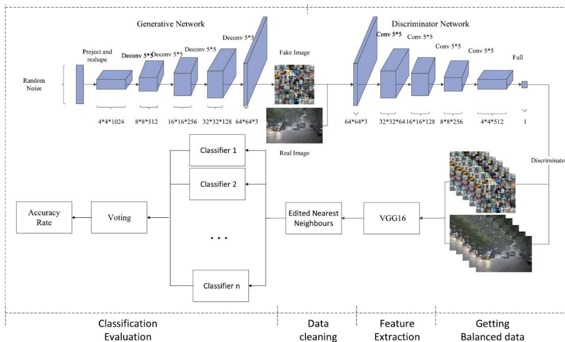
Figure 22: Illustration from Y. Huang et al. [193] showing how the Ensemble learning is integrated with GAN Framework.
