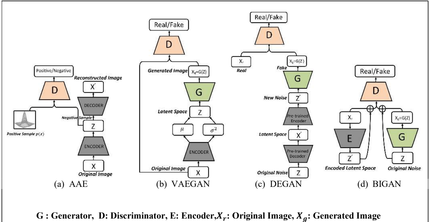
Figure 10: A schematic view of Variants of GANs based on Encoder and decoder architecture: (a) AAE, (b) VAEGAN, (c) DEGAN and (d) BIGAN
