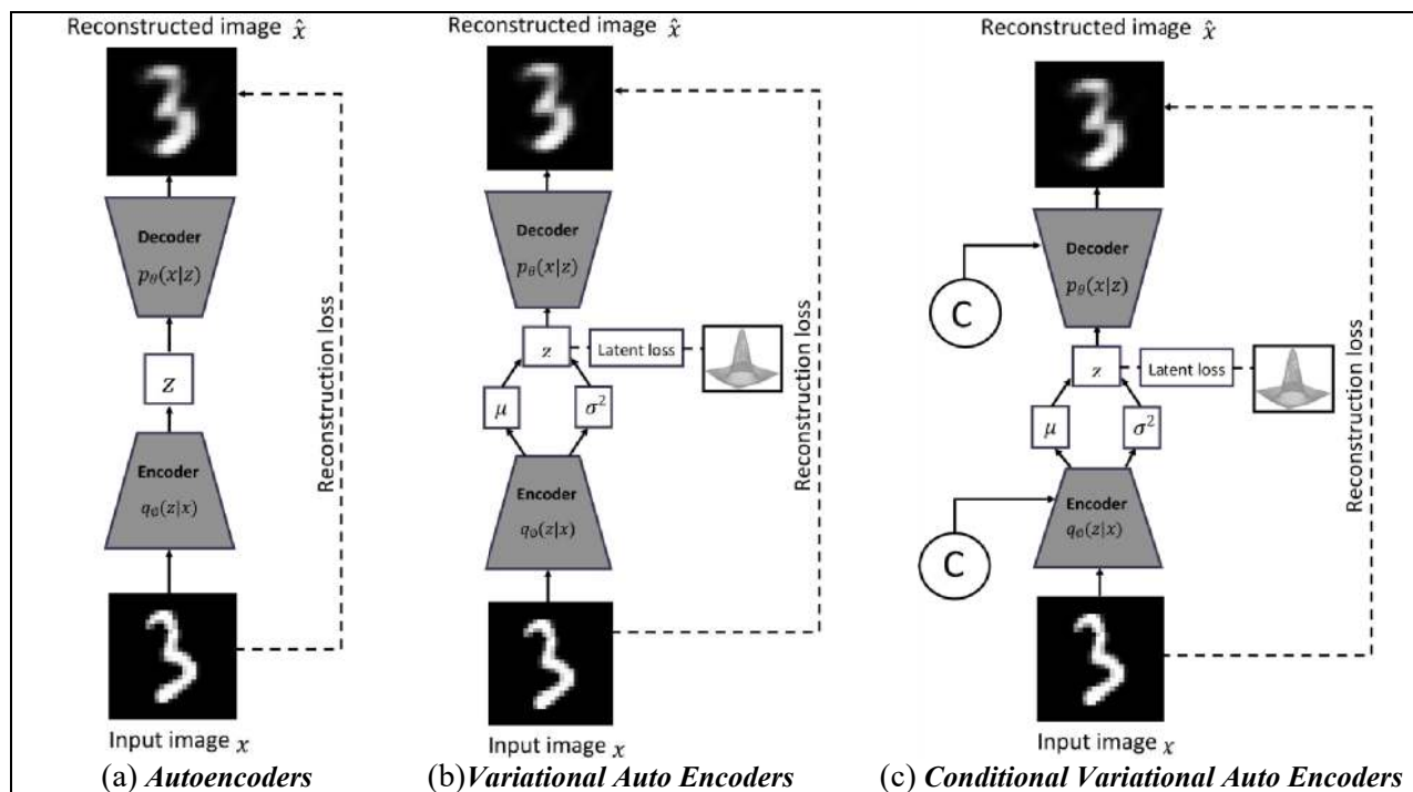
Figure 5: The architecture of (a) Autoencoders; (b) Variational Auto Encoders; (c) Conditional Variational Auto Encoders
