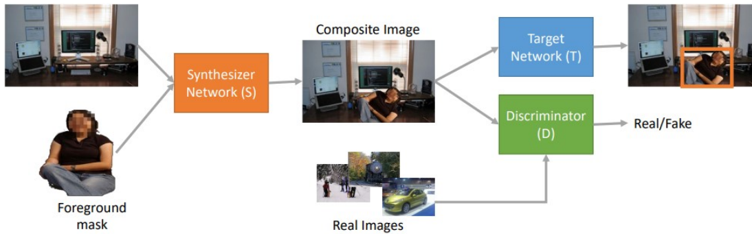
Figure 31: Pipeline of task aware image synthesis used by Tripathi et.al [214]
