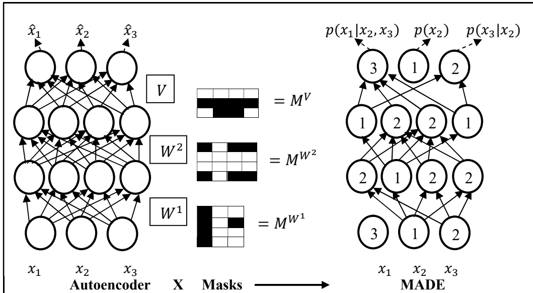
Figure 4: An illustration of Masked Autoencoder Density Estimator (MADE)[92]. A set of connections in an autoencoder is removed using multiplicative binary masks, such that each output unit is connected only to relevant input units.
