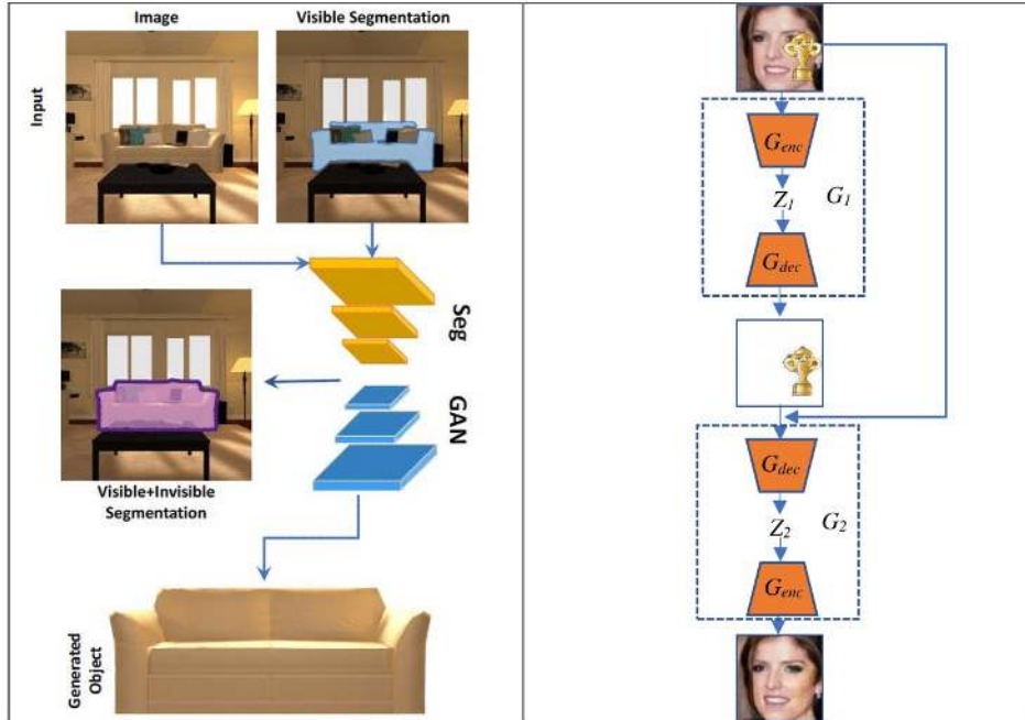
Figure 33: Illustration of SeGAN[226](left) and Occlusion-Aware GAN [227](right)
