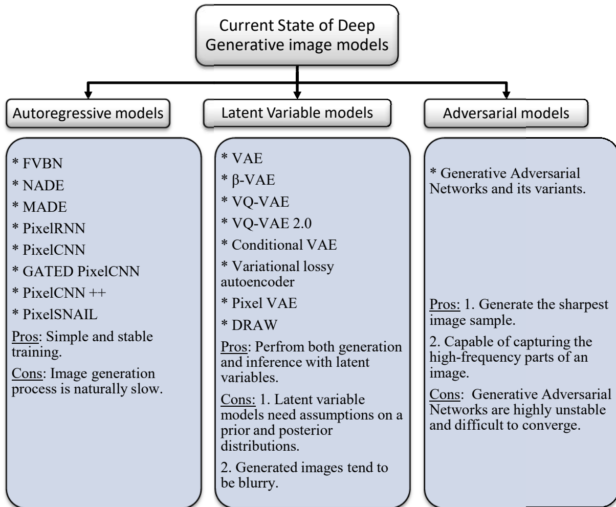
Figure 7: Comparative summary of Deep generative models discussed in section 2.
