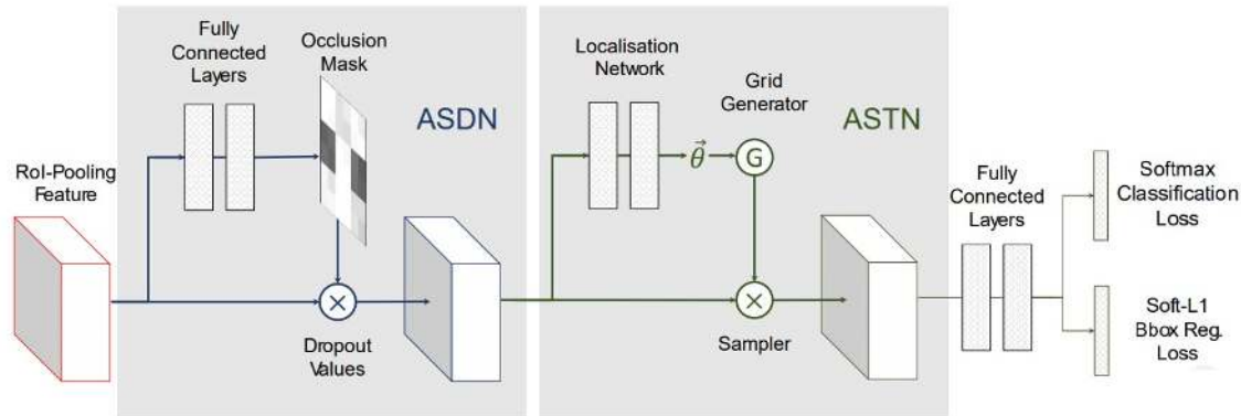
Figure 30: Architecture diagram to generate hard examples for training [211]
