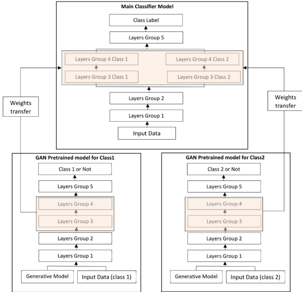
Figure 25: Illustration of the class expert generative adversarial network architecture [200]
