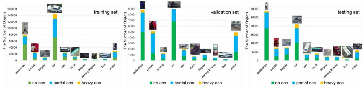
Figure 28: Imbalanced distribution of occluded, partially occluded and heavily occluded objects in VisDrone-DET2018 dataset [210]
