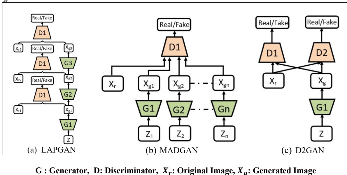
Figure 9: A schematic view of Variants of GANs with multiple discriminators and generators: (a) LAPGAN, (b) MADGAN and (c) D2GAN
