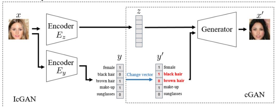
Figure 15: illustration of invertible conditional GAN presented by Perarnau et al. [165]
