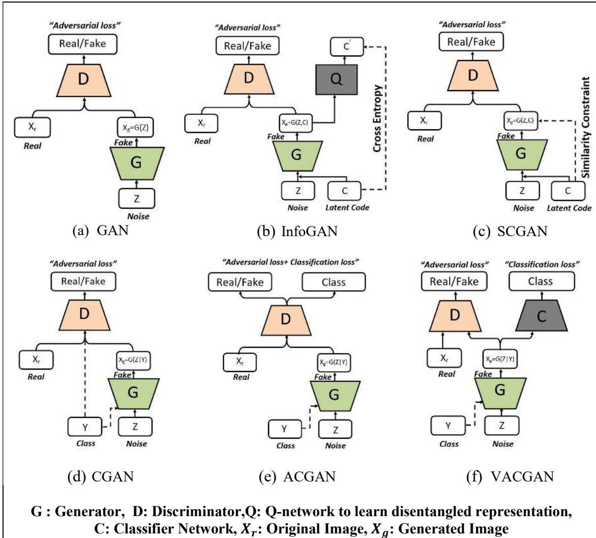
Figure 8: A schematic view of (a) the vanilla GAN and (b)-(f) variants of Conditional GANs
