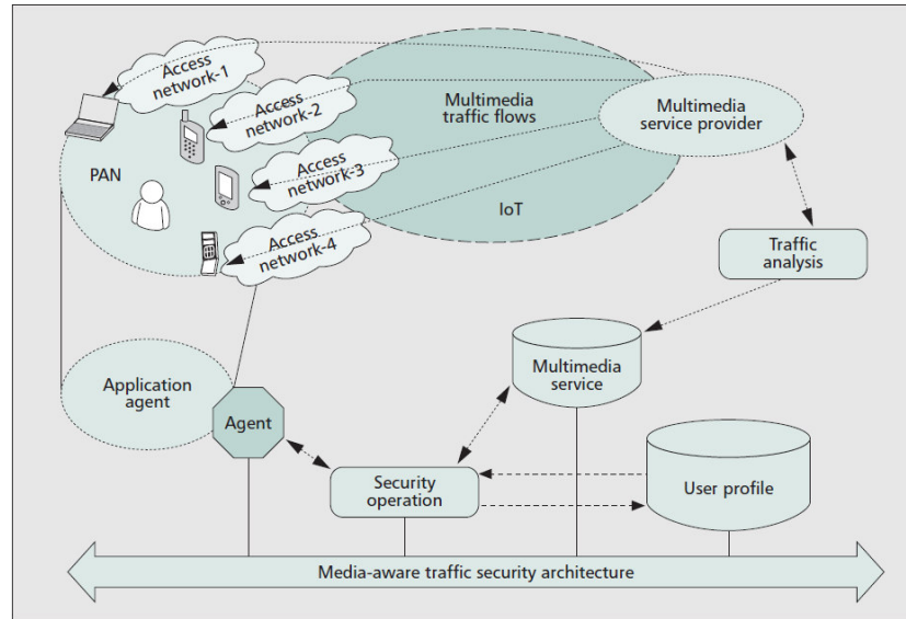
Figure 11. MTSA architecture.
