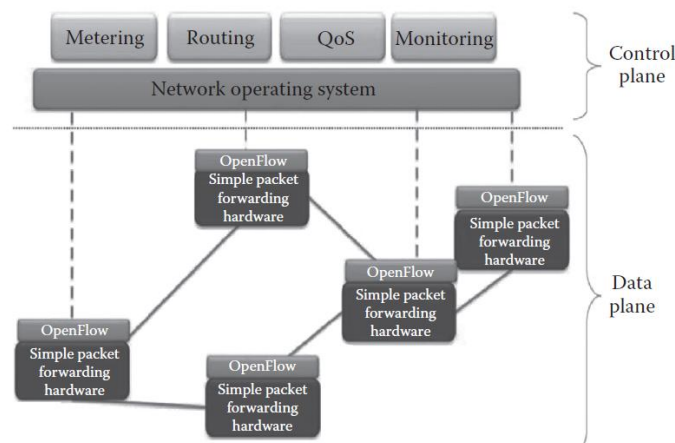
Fig. 1: SDN Architecture [5]
