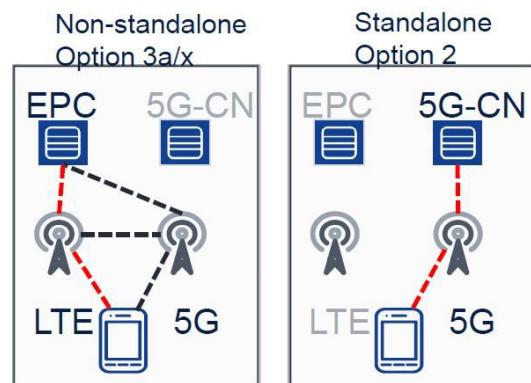
Fig. 5: Proposed 5G architectures in 3GPP Release 15 [31].
