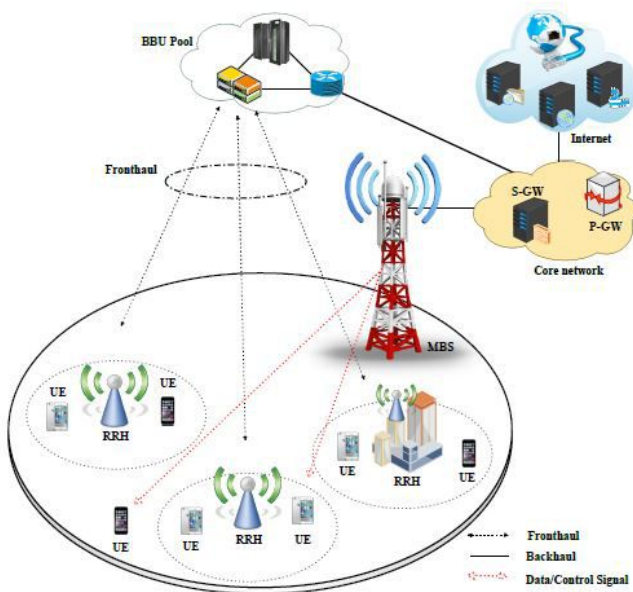
Fig. 6: Schematic of C-RAN architecture [65].
