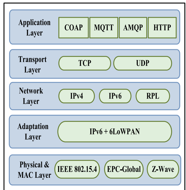
FIGURE 4. Layer structure of the 6LoWPAN.
