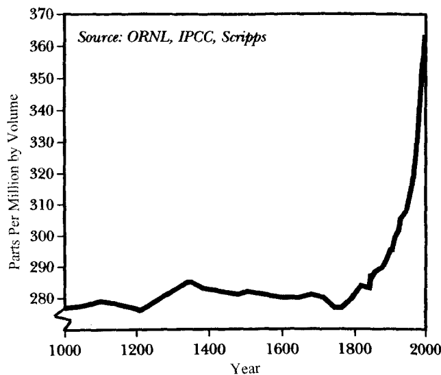
Figure 2 Atmospheric Levels of Carbon Dioxide From 1000 to 1997
