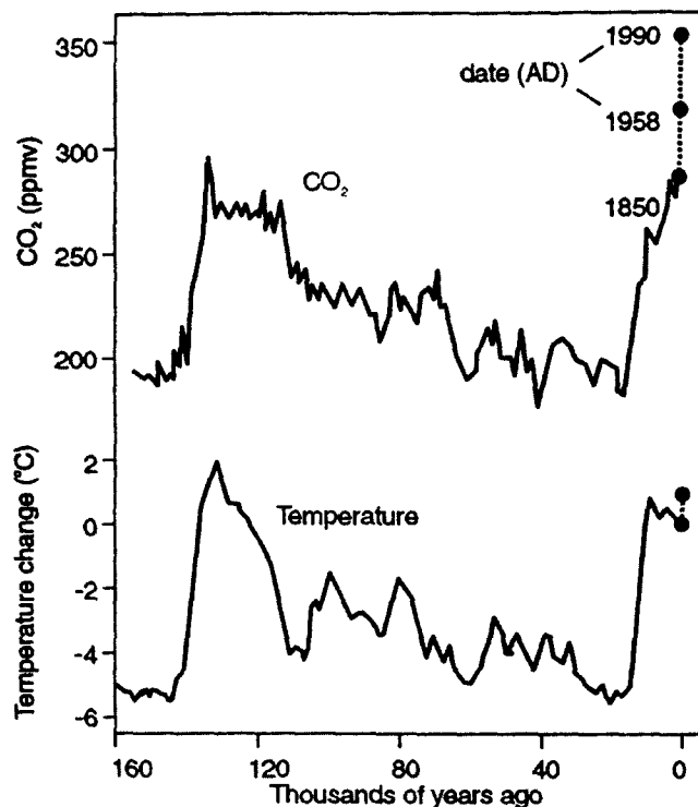
Figure 1 Parallelism of Earth's Atmospheric CO 2 Levels and Temperature Changes Over the Past 160,000 Years
