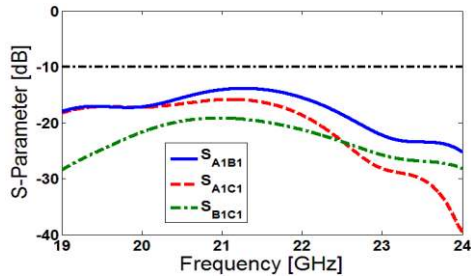
Fig. 7. Mutual couplings for the antenna elements of different sub arrays.
