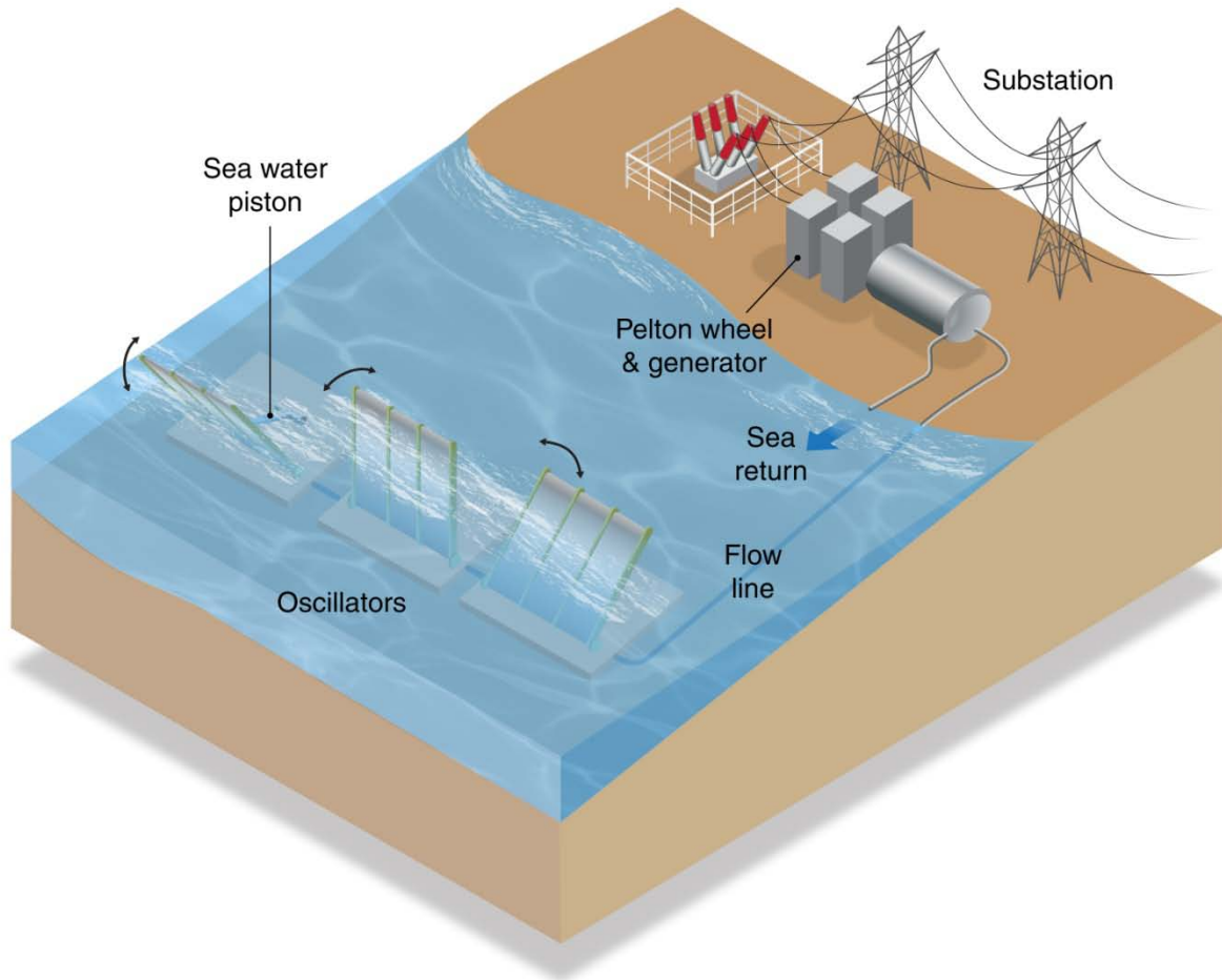
Figure 2. An illustration of the bottom-hinged system. Illustration by AI Hicks, NREL
