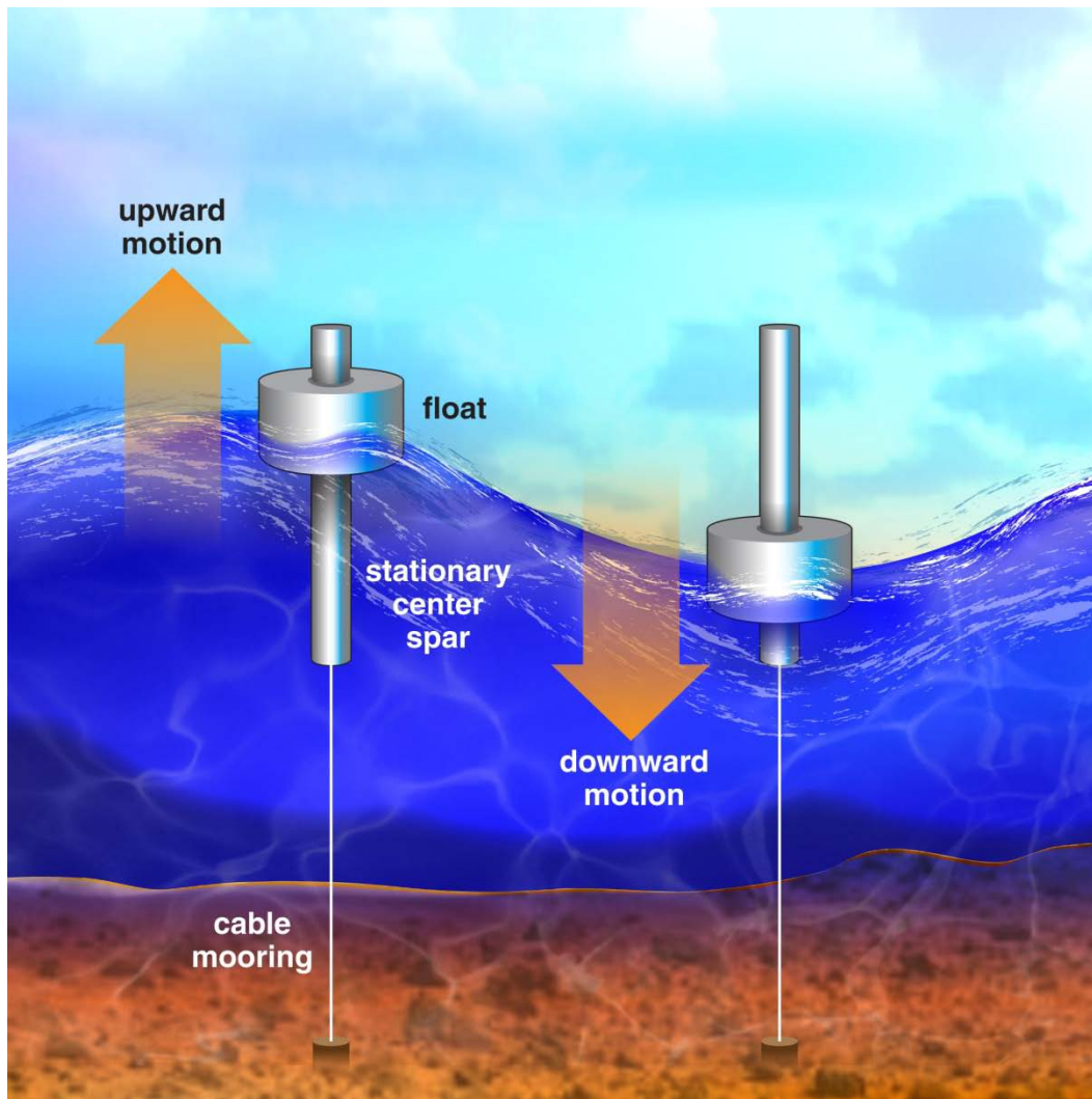
Figure 6. An illustration of the point absorber. Illustration by AI Hicks, NREL
