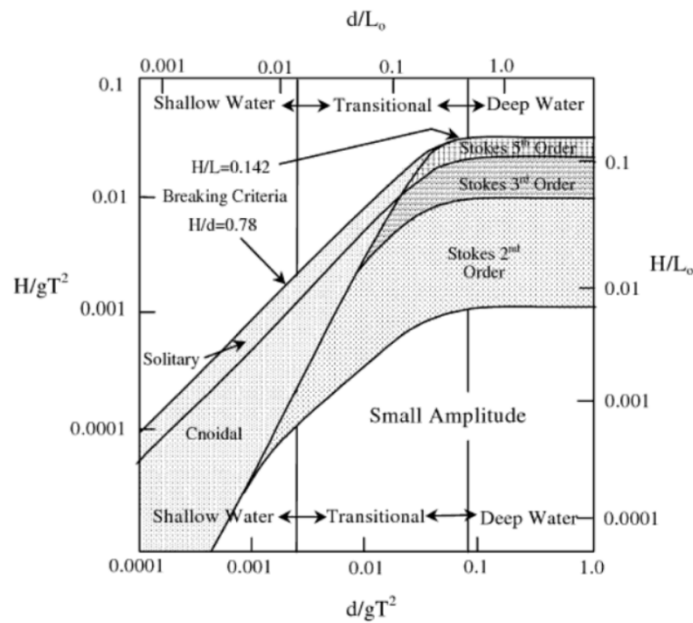
Figure 8. The applicability of various wave theories [44,46]
