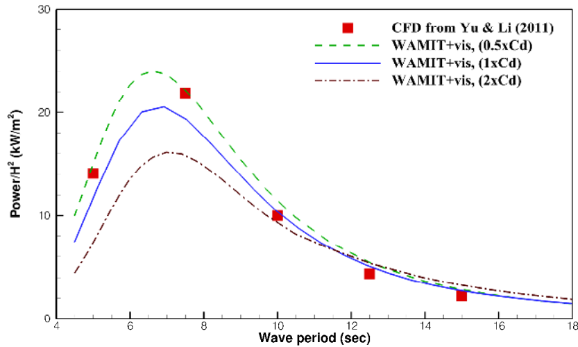
Figure 9. Power generation prediction from NSEM and BIEM ( C_{PT0}=507 \text{ kNsm}^{-1} )
