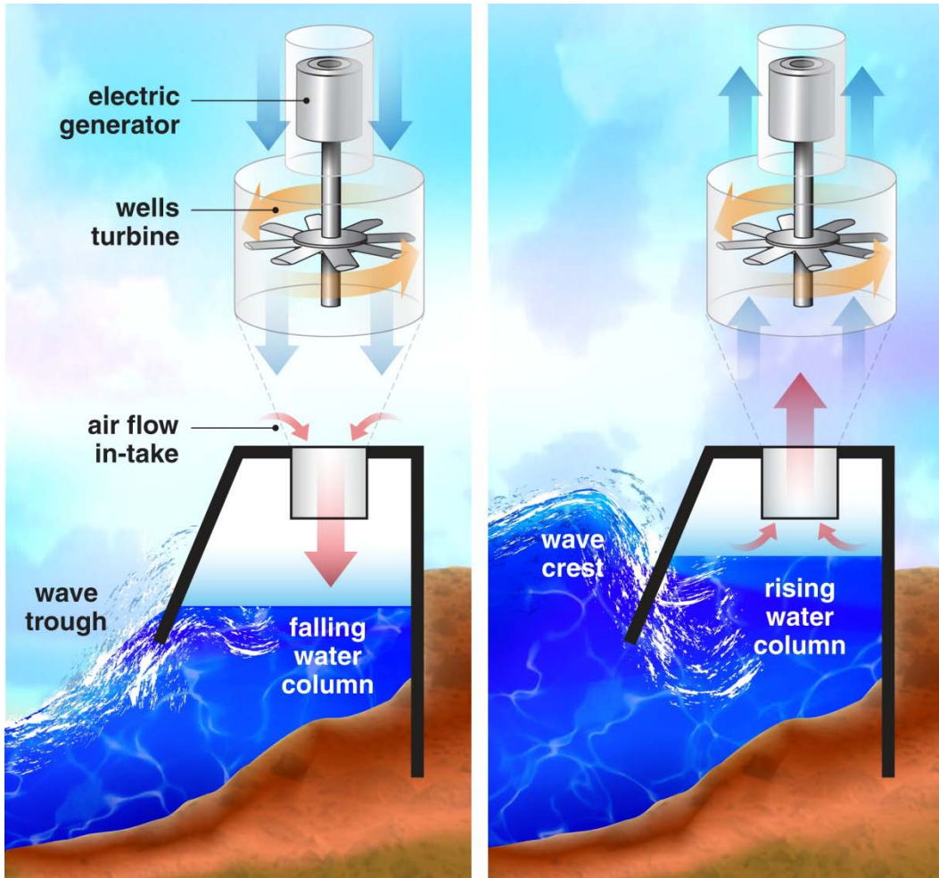
Figure 3. An illustration of the oscillating water column. Illustration by AI Hicks, NREL
