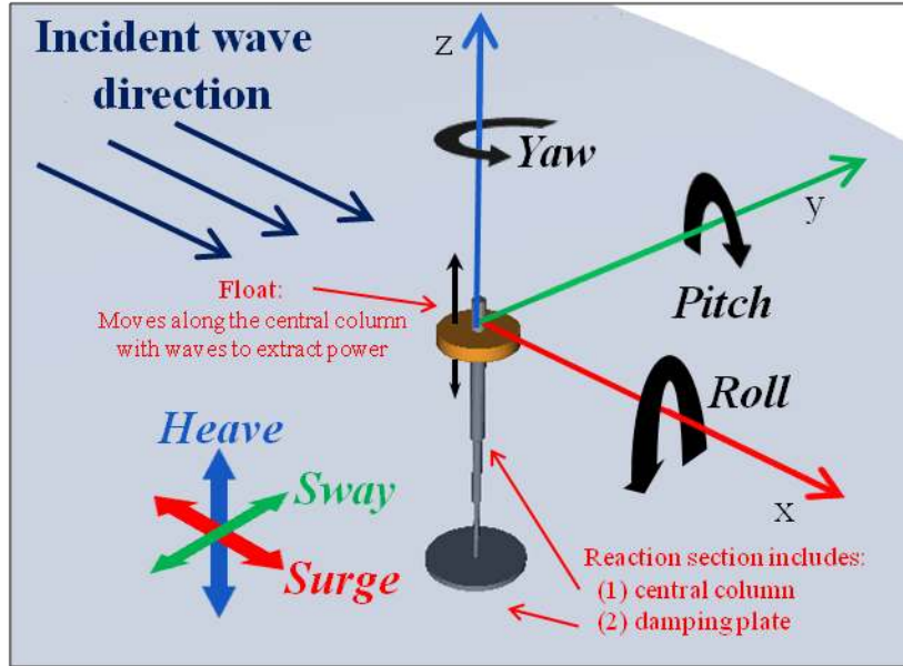
Figure 7. The translation and rotation of the body (6 degrees of freedom)
