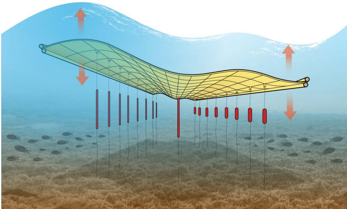
Figure 5. An illustration of the membrane device. Illustration by AI Hicks, NREL
